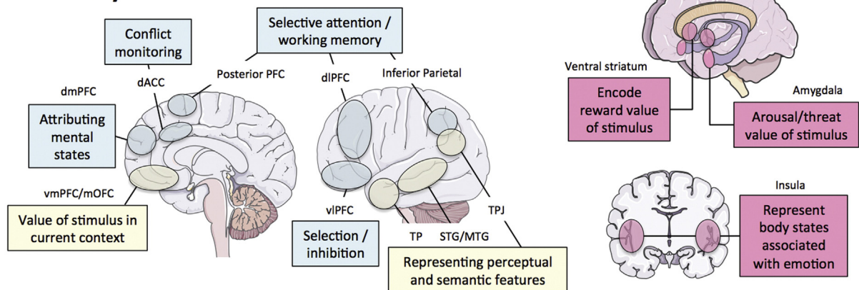
Fig. 1. A model of the cognitive control of emotion (MCCE). (A) Diagram of the processing steps involved in generating an emotion and the ways in which cognitive control processes (blue box) might be used to regulate them. As described in the text, the effects of different emotion regulation strategies (the red arrows descending from the cognitive control processes box) can be understood in terms of the stages of the emotion generation sequence that they influence. The pink box seen at the appraisal stage is meant to indicate that neural systems involved in generating emotion support this process. (B) Neural systems involved in using cognitive strategies, such as reappraisal, to regulate emotion (left, blue boxes), systems involved in generating those responses (left, pink boxes), and systems with an undefined or intermediary role in reappraisal (left, yellow boxes; adapted from Ochsner et al., 2012 with permission). Brain schematic representations were provided by Servier Medical Art ( http://www.servier.fr ).
