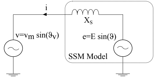
Figure 3. Model of an SSM connected to the grid.
