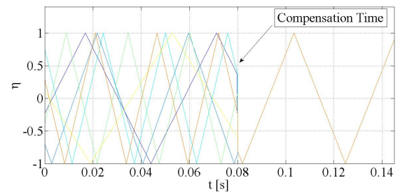
Figure 19. The PWM modulation waveform signals of the six node with decentralized topology, with t_{del} = 10^{-4} s
