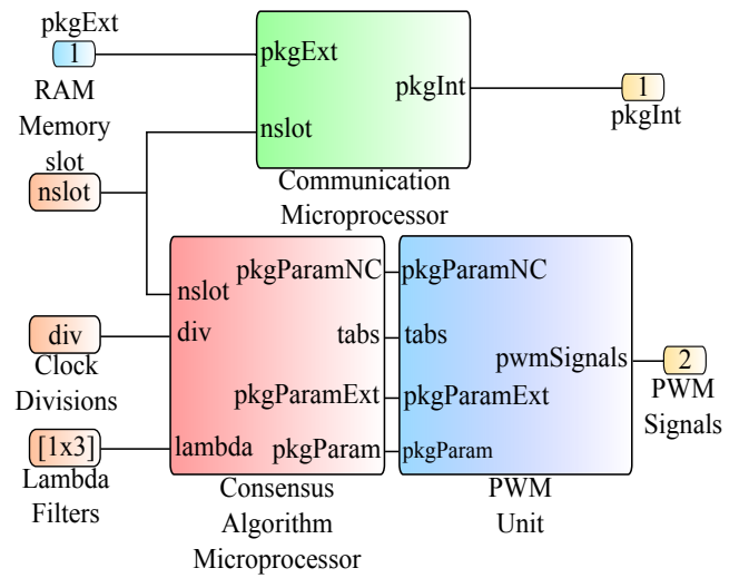
Figure 8. The single Agent developed in Matlab/Simulink ® .
