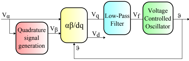
Figure 2. SRF-PLL for single-phase signals.
