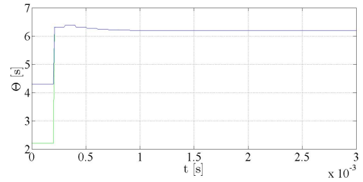
(a) With t_{del} = 0 s.
