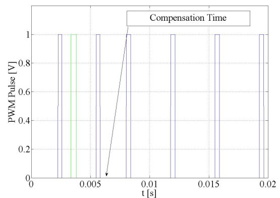
(b) With t_{del} = 10^{-4} s.
