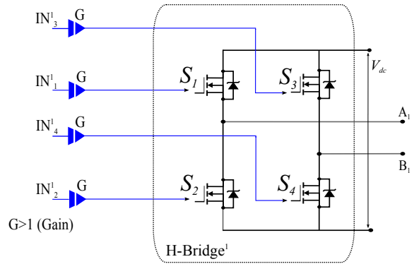
(b) Detail of H-Bridge 1 .
