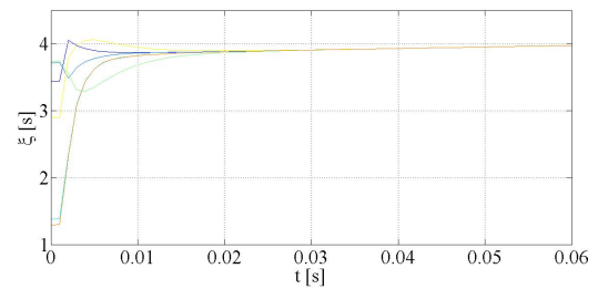
(b) The six clocks convergence dynamics, with t_{del} = 10^{-4} s.
