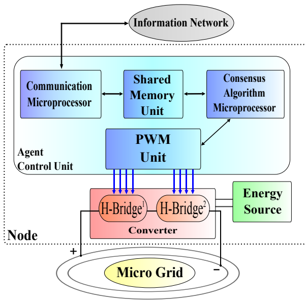
Figure 7. The ACU detail.
