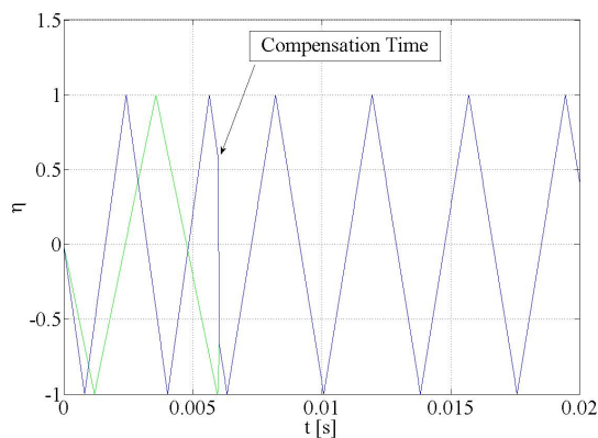
(b) With t_{del} = 10^{-4} s.
