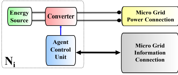
Figure 5. The generic node N_i and its subsystems: the energy source, the power converter and the ACU.
