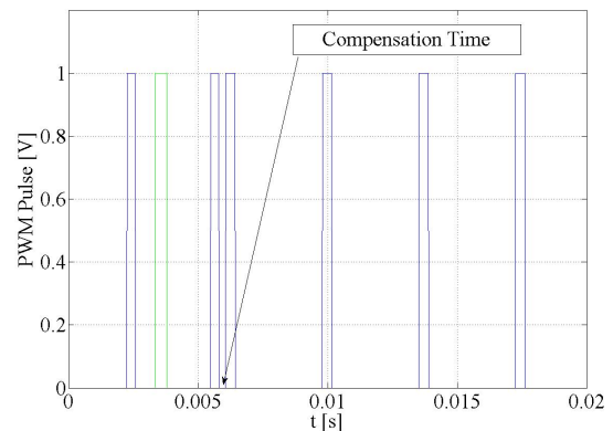
(a) With t_{del} = 0 s.
