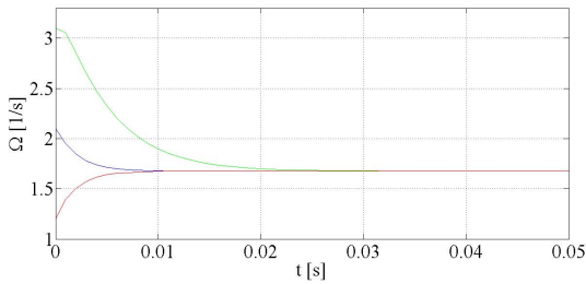
(a) The three clocks skew convergence, with t_{del} = 10^{-4} s
