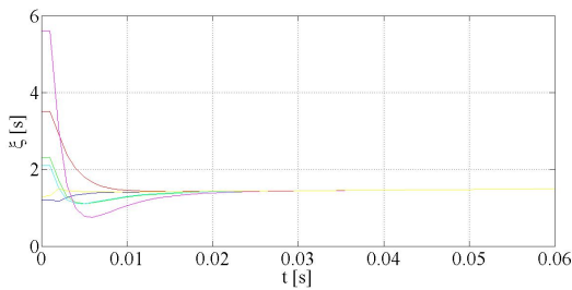
(b) The six clocks convergence dynamics, with t_{del} = 10^{-4} s.
