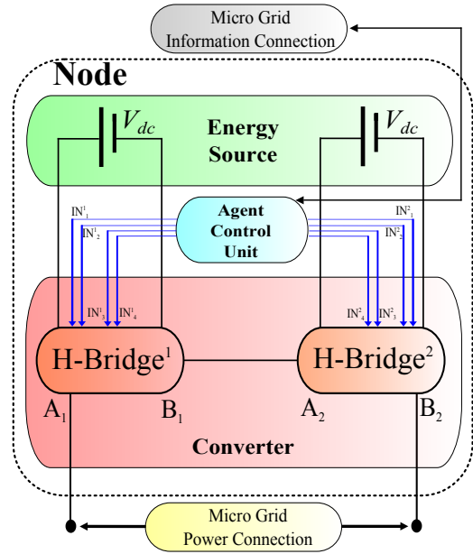
(a) Cascaded H-bridge 5-level converter.
