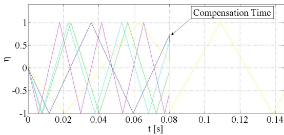
Figure 17. The PWM modulation waveform signals of the six node with centralized topology, with t_{del} = 10^{-4} s
