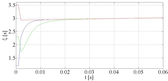
(b) The three clocks convergence dynamics, with t_{del} = 10^{-4} s .
