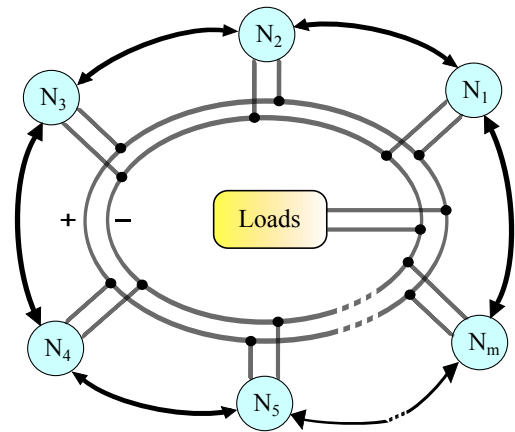
Figure 4. Microgrid: grey lines represent Power Grid, black arrows represent Information Network, circles represent nodes.
