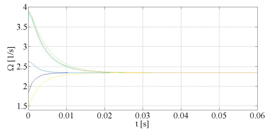
(a) The six clocks skew convergence, with t_{del} = 10^{-4} s
