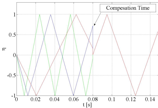
Figure 14. The PWM modulation waveform signals of the three nodes, with t_{del} = 10^{-4} s
