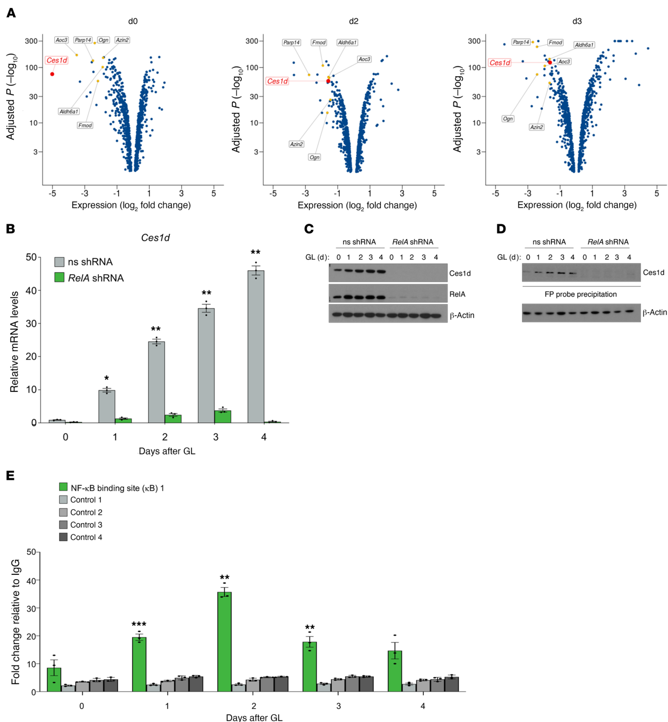
Figure 3. Ces1d is a direct transcriptional target of NF- \kappa B and one of the top 7 genes upregulated by NF- \kappa B during starvation. (A) Volcano plots showing differentially expressed metabolic genes ( q < 0.05 ; d0, n = 801 ; d2, n = 726 ; d3, n = 833 ) in RelA -deficient relative to control MEFs ( n = 5 ) cultured under normal conditions (d0) or for 2 (d2) or 3 (d3) days under GL. Reported are the negative \log_{10} -transformed adjusted P values plotted against the average \log_2 fold changes. Dots represent individual genes. Ces1d is depicted as a red dot; the other 6 most markedly downregulated metabolic genes in RelA -deficient relative to control MEFs, across all time points investigated, are depicted as orange dots. (B) qRT-PCR showing the Ces1d mRNA levels in CT-26 cells expressing RelA -specific or ns shRNAs and cultured under normal conditions (0) or for the indicated times under GL. Values denote mean \pm SD ( n = 3 ). (C) Western blots showing the protein levels of Ces1d , RelA , and \beta -actin in CT-26 cells from B . (D) Desthiobiotin-fluorophosphonate activity-based (FP) probe precipitation assays showing the Ces1d -specific serine esterase activity in CT-26 cells from B , as determined by streptavidin-mediated precipitation of the biotin-bound FP probe followed by Western blots with anti- Ces1d antibody. \beta -actin in the total cell lysates (input) used for the activity-based protein profile (ABPP) assay is shown as a loading control. (E) Chromatin immunoprecipitation assays showing the binding of NF- \kappa B/ RelA complexes to \kappa B DNA element 1 ( \kappa B1) in the promoter region of Ces1d or the indicated control DNA regions (controls 1–4) in CT-26 cells from B . Values denote mean \pm SEM ( n = 3 ). (B–E) Experiments were conducted at least 3 times. (B and E) Statistical significance was calculated by 2-tailed Student's t test. * P < 0.05 ; ** P < 0.01 ; *** P < 0.001 .
