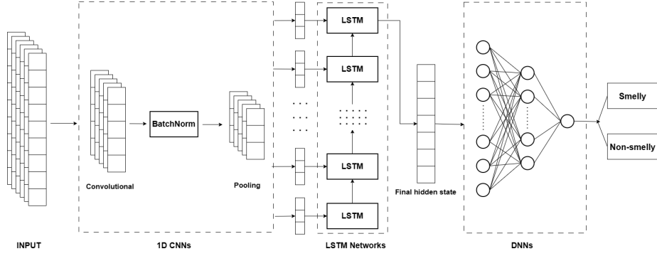
Figure 1: The overall DEEPSMELLS architecture.
