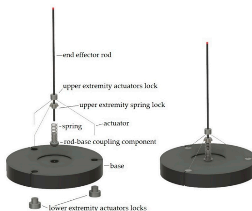
Figure 8. The CAD model of the manipulator.
