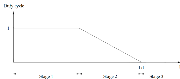
Figure 10. Control logic scheme: in stage 1, far from the target, the control supplies the maximum power. In stage 2, close to the target, the control becomes proportional. At stage 3, overcoming the target, the control cuts power off.
