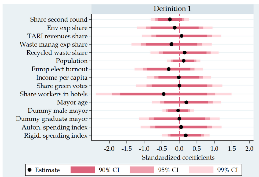
Fig. 1. Balance test of covariates at the margin (Definition 1).
