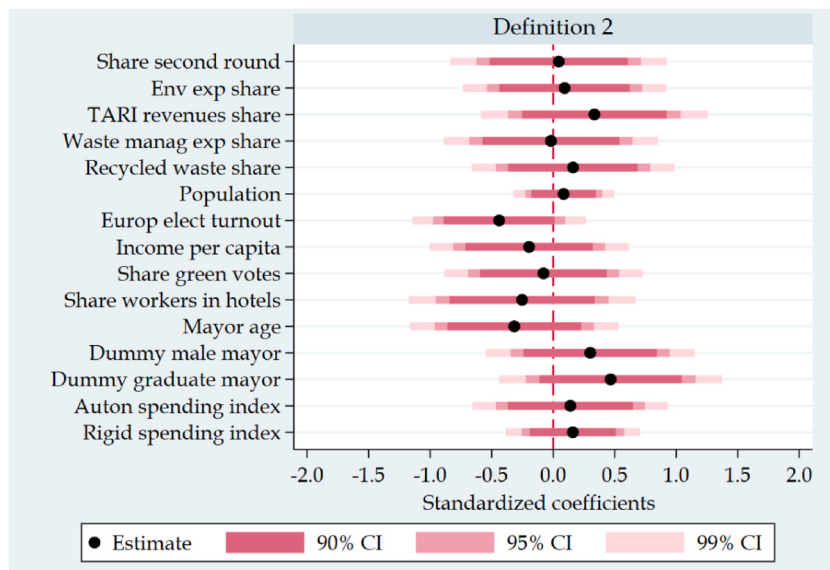
Fig. A.1. Balance test of covariates at the margin (Definition 2). notes: See notes of Fig. 1.
