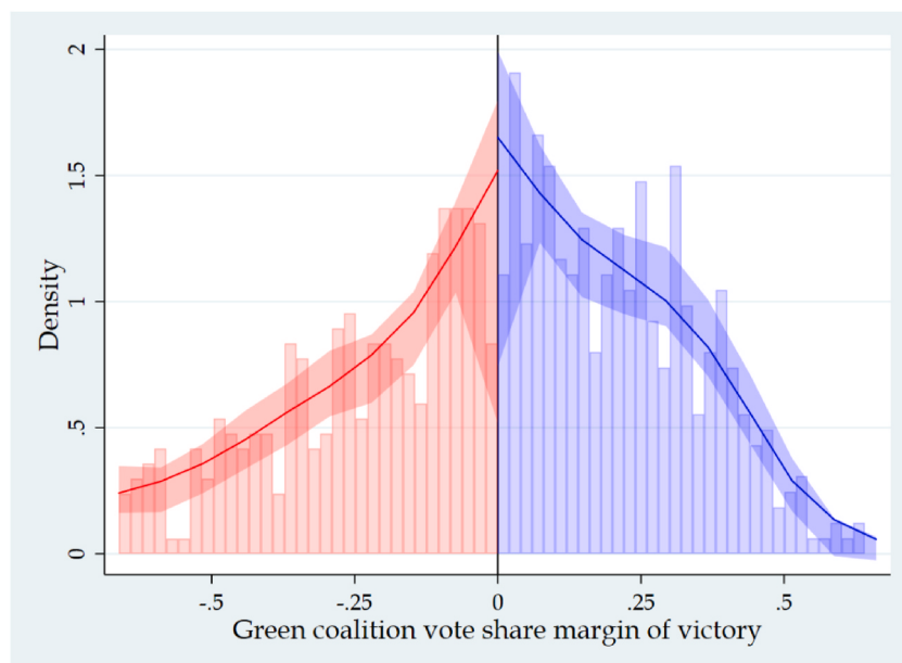
Fig. A.4. Manipulation testing plot (Definition 3).
