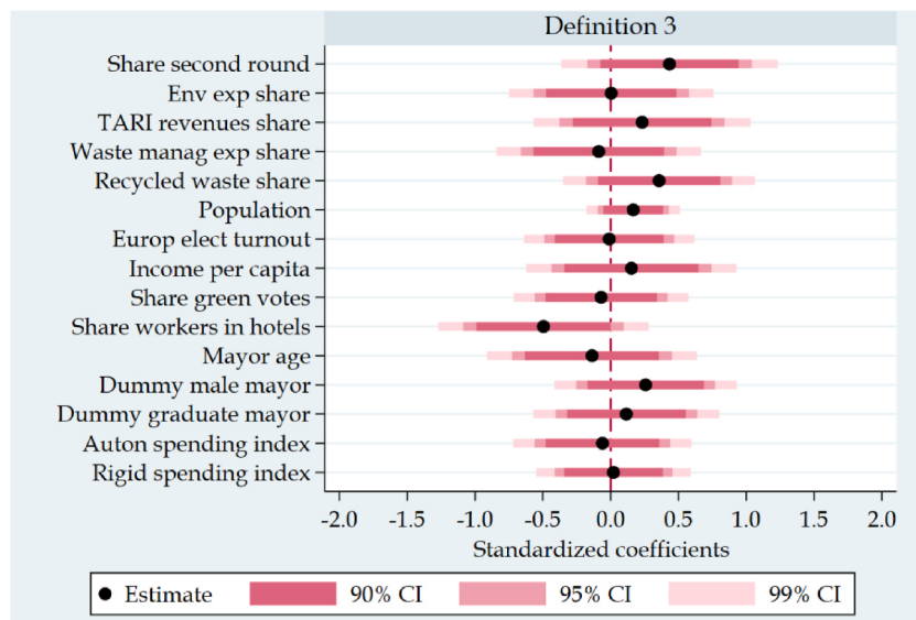
Fig. A.3. Balance test of covariates at the margin (Definition 3).
