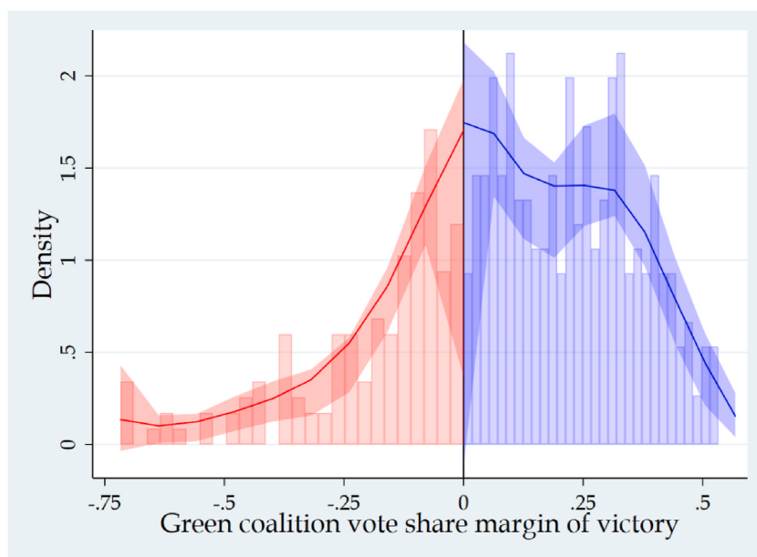
Fig. 2. Manipulation testing plot (Definition 1).
