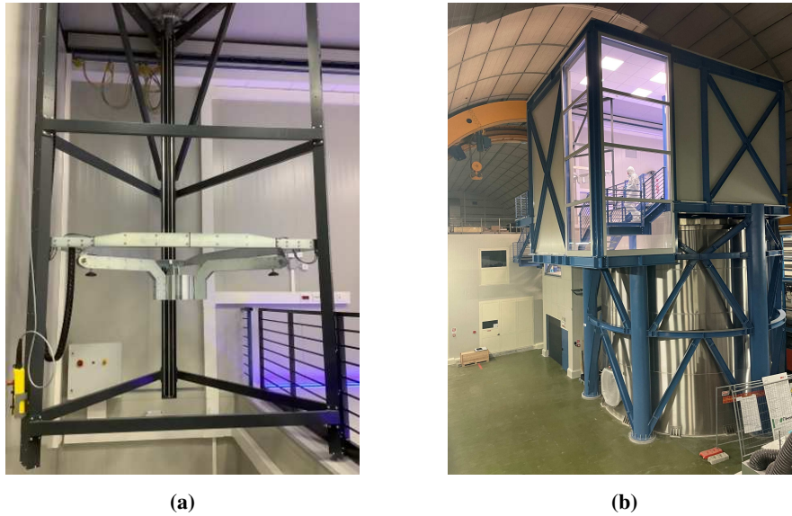
Figure 4: The lifting system in the maintenance bay inside the clean room a and the clean room as seen from outside b . The lifting frame is the metal piece in the middle of the painted truss seen in a . The lifting system can be seen in the background in b . Inside the windows the maintenance bay can be seen.
