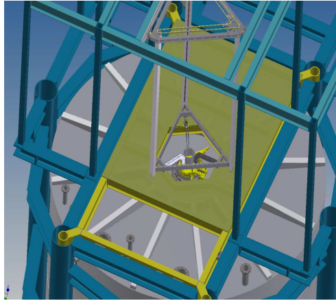
Figure 2: A rendering of the two frames of the experiment as seen from above. The two frames (in blue and yellow) are decoupled, while the water tank is shown in grey.
