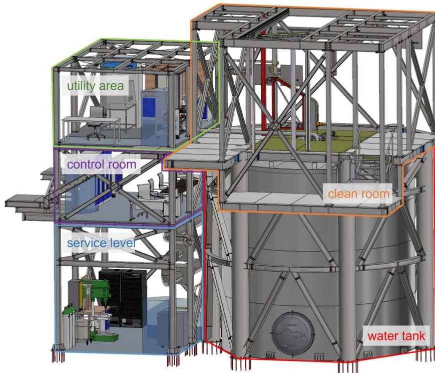
Figure 1: A CAD drawing of the experimental facility. The refrigerator will be inside the water tank that is outlined in red. The region above the water tank outlined in orange is the ISO 6 level clean room. This is where the cryostat will be moved to when the detectors are installed into the cryostat.
