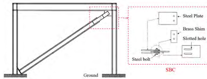
Figure 1. Example of structure fitted with a slotted bolted connection (SBC) with steel–brass sliding surfaces.
