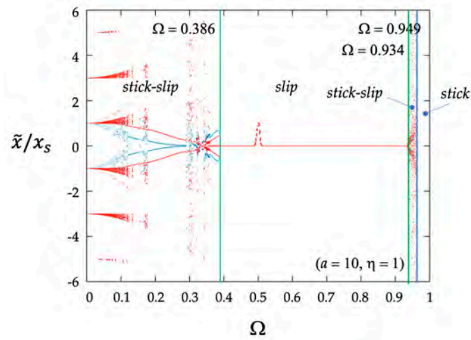
Figure 8. Bifurcation diagrams in the domain \Omega - \tilde{x}/x_s for a = 10 and \eta = 1 . Blue points on the diagram correspond to sticking phase, red points are associated with sliding phase.
