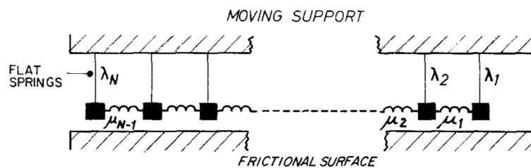
Figure 3. Schematic representation of the Burridge–Knopff model (figure drawn from [1]).
