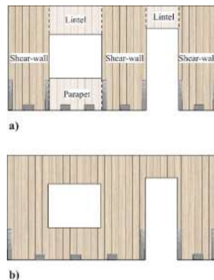
Figure 1. a) Monolithic (MSW) shear wall, b) Segmented (SSW) shear wall Fracture modes
