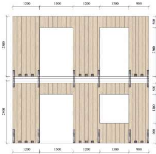
Figure 10: Shear-wall Configuration #2 (measures in mm)
