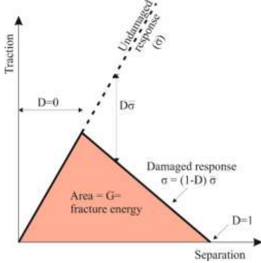
Figure 3. Damage initiation and evolution
