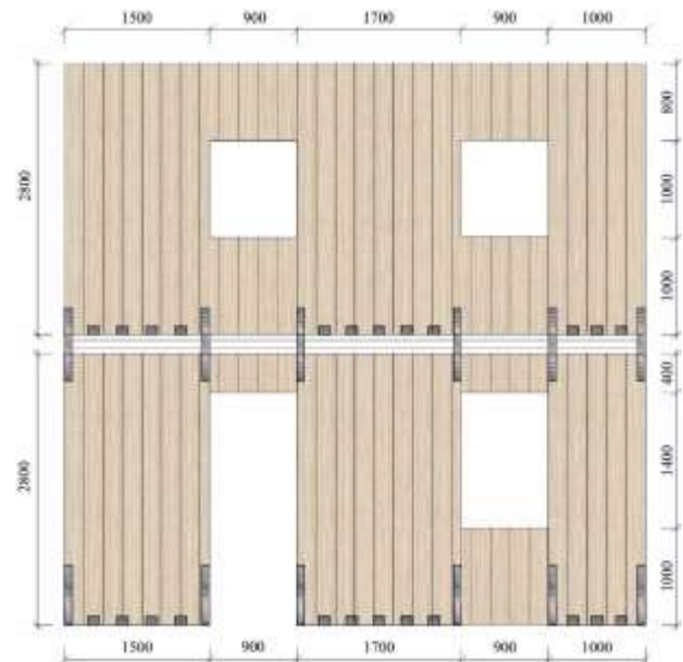
Figure 9: Shear-wall Configuration #1 (measures in mm)
