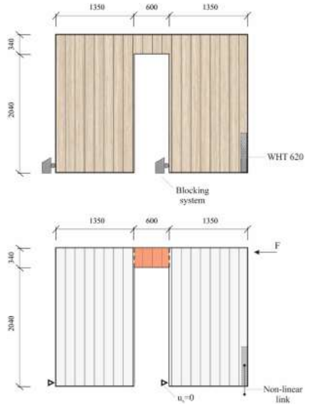
Figure 5: Wall 1: Test setup (top) and schematic plan of partitions and mechanical anchors definition in Abaqus models (bottom) (measures in mm)
