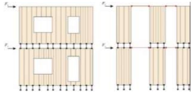
Figure 8: left) MSW model; right) SSW model
