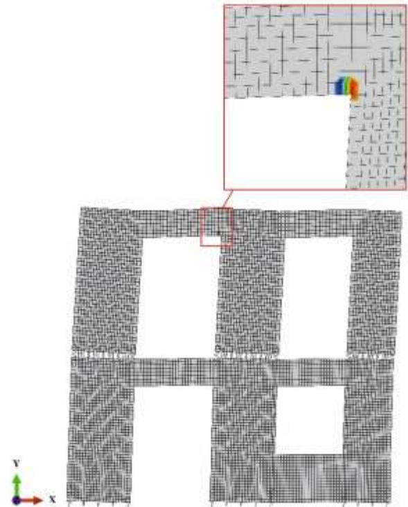
Figure 13: Fracture mechanisms for Configuration #2.
