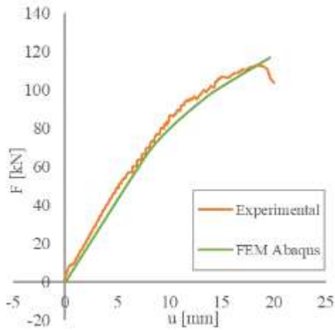
Figure 6. Model validation with crack opening
