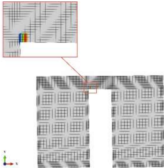
Figure 7. Model validation with crack opening
