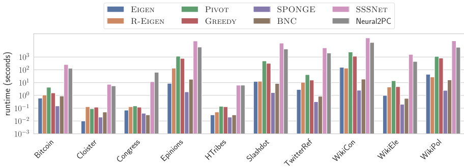
Fig. 5 Execution times (in seconds) of the proposed Neural2PC method vs. competing methods on real-world network datasets
