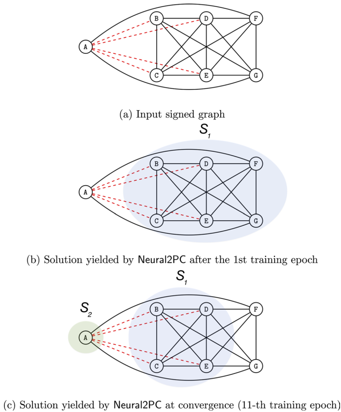
Fig. 4 Running example illustrating a scenario of node-isolation detection (Example 3)
