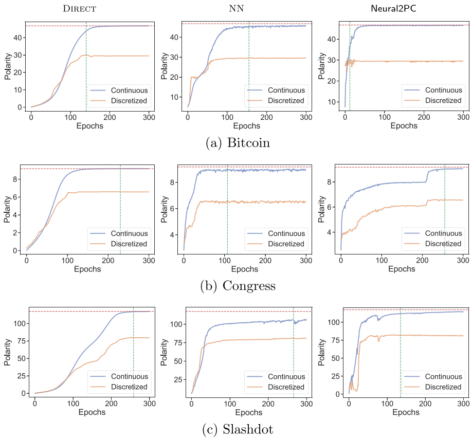
Fig. 7 Polarity scores by varying the number of epochs, for Neural2PC and its simplifications relevant to the ablation study (i.e., DIRECT and NN). Each plot distinguishes between polarity of the continuous (i.e., relaxed) solution and polarity of the discretized (i.e., rounded) solution. Green vertical lines correspond to peaks of the rounded solutions' polarity, while top red horizontal lines set the upper-bound of polarity (i.e., polarity of the optimal (relaxed) solution to the 2PC-RELAXED instance on a particular graph)
