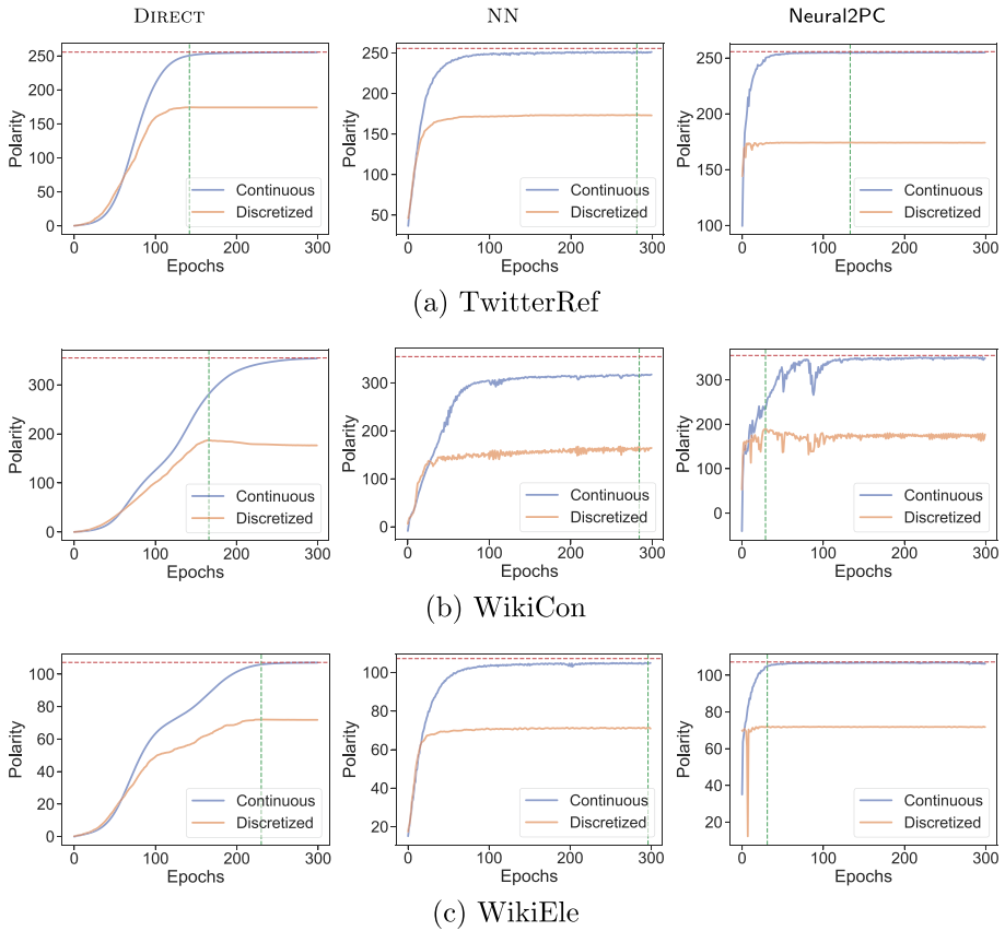
Fig. 8 (Cont.) Polarity scores by varying the number of epochs, for Neural2PC and its simplifications relevant to the ablation study (i.e., DIRECT and NN). Each plot distinguishes between polarity of the continuous (i.e., relaxed) solution and polarity of the discretized (i.e., rounded) solution. Green vertical lines correspond to peaks of the rounded solutions' polarity, while top red horizontal lines set the upper-bound of polarity (i.e., polarity of the optimal (relaxed) solution to the 2PC-RELAXED instance on a particular graph)
