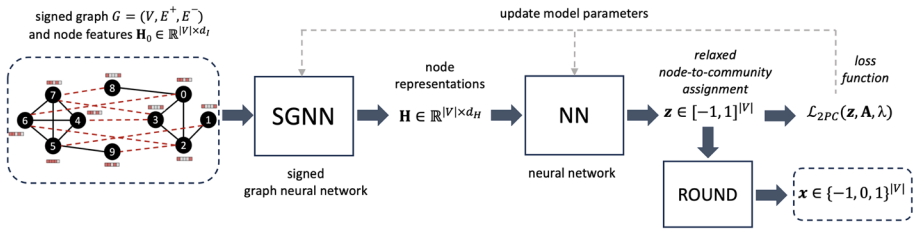
Fig. 2 Overview of the proposed Neural2PC approach
