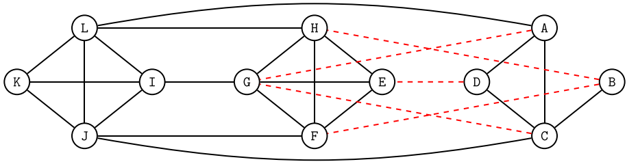
Fig. 3 Example signed graph where, unlike basic polarity, \gamma -polarity detects effective polarized communities that are also size-balanced (Example 2)
