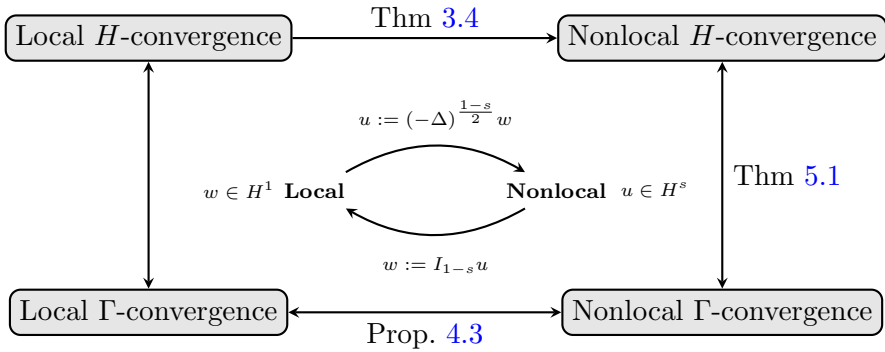
Fig. 1 The relations between H - and \Gamma -convergence in the case of symmetric matrices in the local and nonlocal scenarios.
