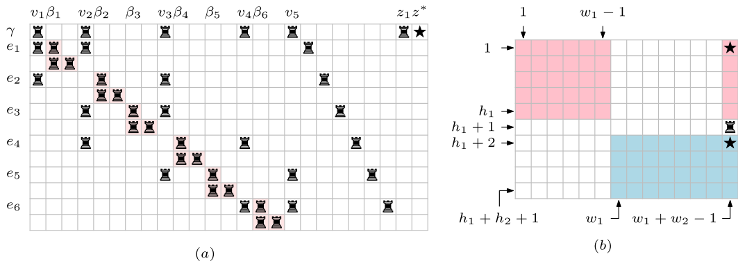
Fig. 14. (a) The instance of \text{SOLO-CHESSE}^*(\mathbb{N}, \{2\}) by applying our transformation to the instance of \text{SOLO-CHESSE}^*(\mathbb{N}, \{0, 2\}) of Fig. 12 (c). Red squares contain the 2-rooks replacing the original 0-rooks. (b) A sketch of the instance \mathcal{I}_{1,2} of \text{SOLO-CHESSE}(\mathbb{N}, \{2\}) obtained from the instances \mathcal{I}_1, \mathcal{I}_2 of \text{SOLO-CHESSE}^*(\mathbb{N}, \{2\}) .
