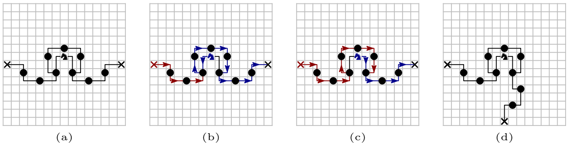
Fig. 3. (a) The arrangement of knights in a straight edge gadget. (b) A sequence of moves that allows the gadget to output a 3-knight from the right I/O square when a 3-knight is input in the left I/O square. Red moves are played before blue moves. (c) A sequence of moves that allows the gadget to output a 7-knight from the right I/O square when a 7-knight is input in the left I/O square. (d) The arrangement of knights in a corner edge gadget. (For interpretation of the references to colour in this figure legend, the reader is referred to the web version of this article.)
