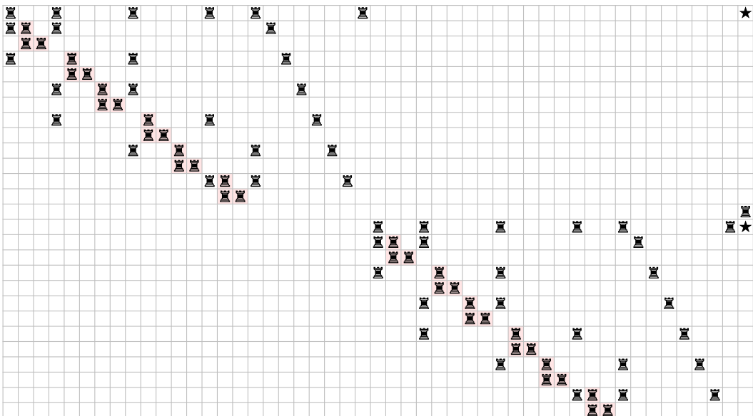
Fig. 15. The final instance \text{SOLO-CHESSE}(\mathbb{R}, \{2\}) corresponding to the vertex cover instance of Fig. 12 (a).
