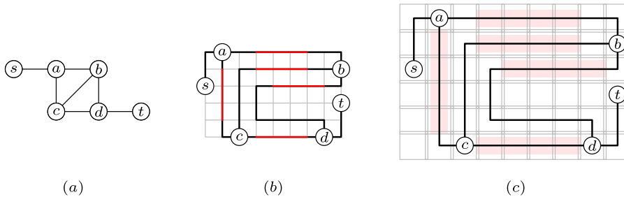
Fig. 1. (a) An instance G of RHP. (b) The corresponding planar orthogonal grid drawing \mathcal{D} of G , where the segments \mathfrak{S}_{u,v}^i are shown in red. (c) A sketch of the chessboard obtained from \mathcal{D} , where the tiles corresponding to the segments \mathfrak{S}_{u,v}^i are highlighted with a red band along the direction of the segment. (For interpretation of the references to colour in this figure legend, the reader is referred to the web version of this article.)
