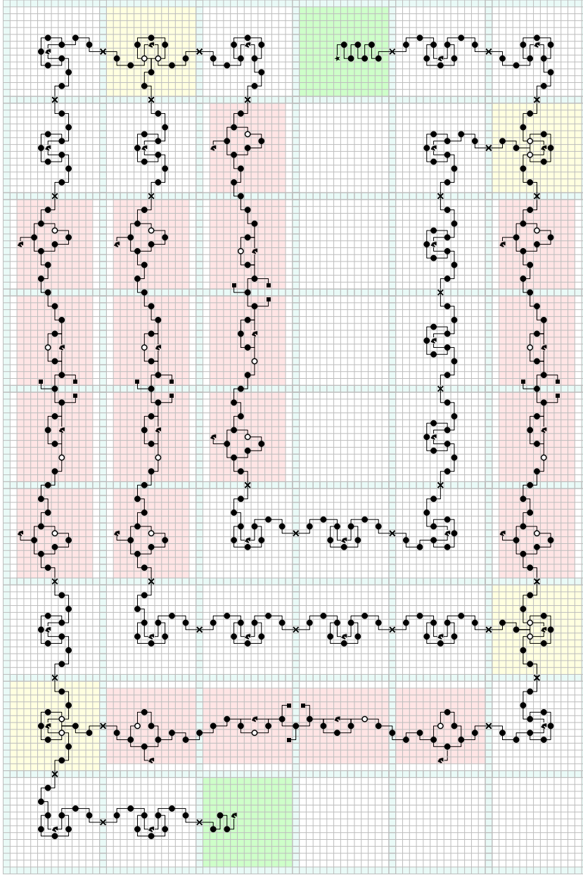
Fig. 7. The chessboard resulting by reducing the instance RHP shown in Fig. 1 (a) to \text{SOLO-CHESSES}(\blacktriangle, \{0, 2, 11\}) . The start, end, edge deletion, and cubic vertex gadgets are highlighted in green, red (with a white border to aid readability), and yellow, respectively. (For interpretation of the references to colour in this figure legend, the reader is referred to the web version of this article.)
