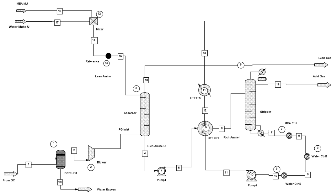
Fig. 2. Layout of the CO 2 capture plant
