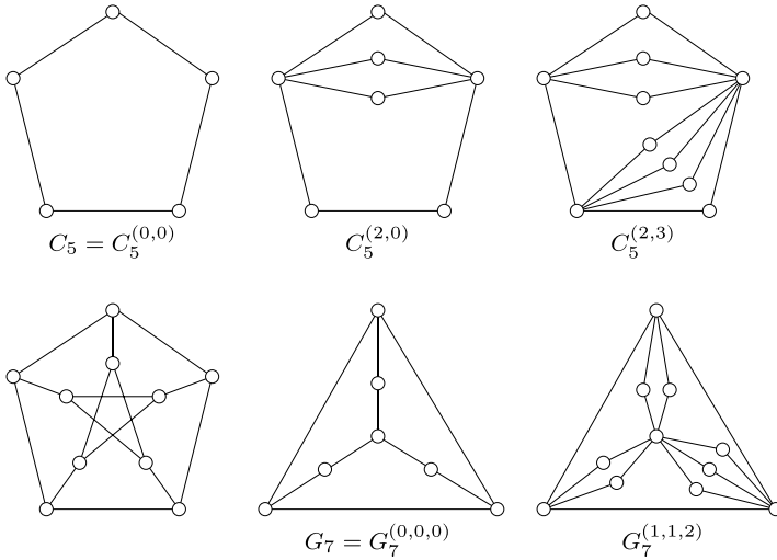
Fig. 3. Some examples of graphs from the family \mathcal{G} .
