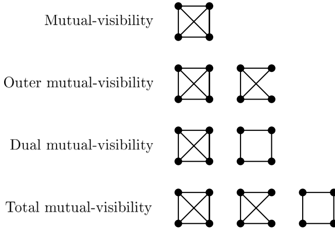
Fig. 2. Forbidden induced subgraphs for (K_n)_F , where F is such that S_F is a (outer, dual, total) mutual-visibility set of L(K_n) .
