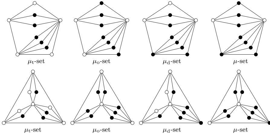
Fig. 4. Variations of mutual-visibility sets in some graphs of the family \mathcal{G} .
