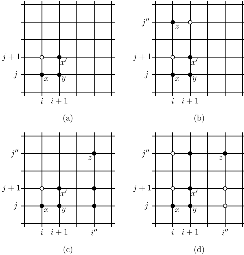
Fig. 1. Cases from the proof of Theorem 2.1(i).
