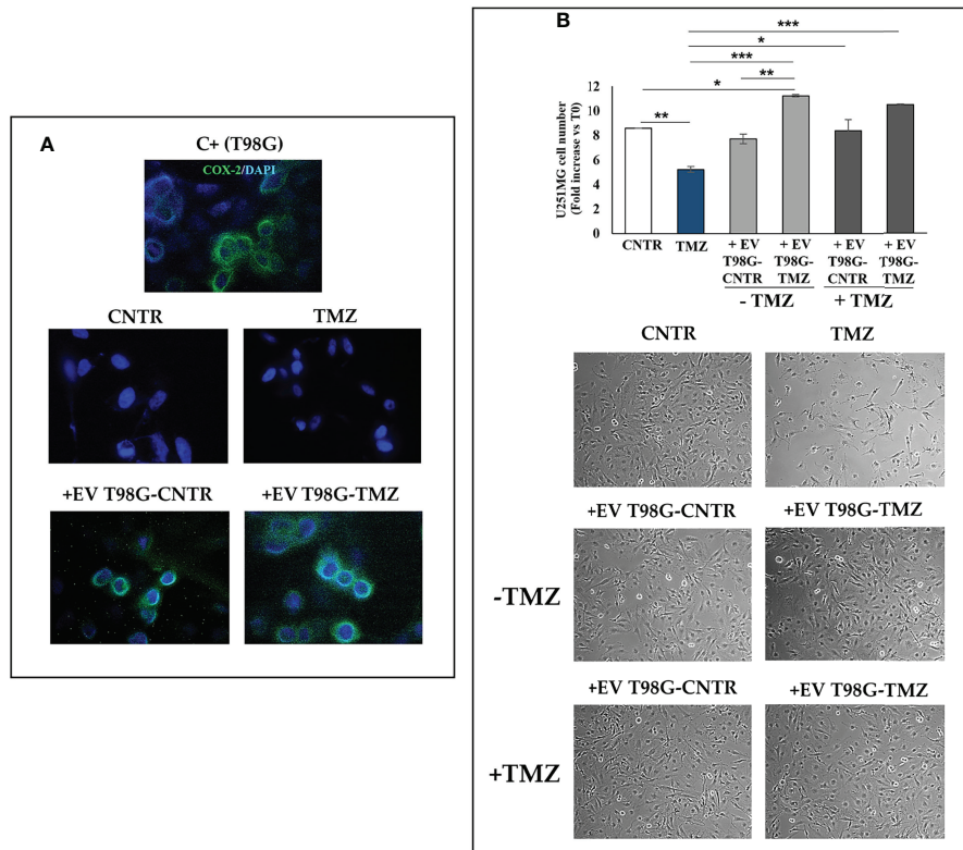
FIGURE 8 | Effect of EV released from TMZ-treated T98G cells on U251MG TMZ-sensitive cells. The U251MG cells were incubated in presence or absence (CNTR) of TMZ (10 \mu M) or with 30 \mu g/ml EV derived from T98G treated with or without TMZ (10 \mu M) for 5 days. (A) Representative immunofluorescence images of U251MG cells treated or not as above described and stained with anti-COX-2 antibody (green) from one out of two independent experiments are shown. Nuclei were counterstained with DAPI (blue). T98G cells are used as positive control (C+). All images were acquired at 100 \times magnification. (B) Cell number was recorded by Trypan blue staining and representative images were taken at 10 \times magnification. All values are given as fold increase vs. initial time (T0). The results, derived from three experiments performed in duplicate, are expressed as mean \pm SEM. For comparative analysis of data groups, a one-way ANOVA with Tukey post hoc test was used (* P <0.05; ** P <0.01; *** P <0.001).
