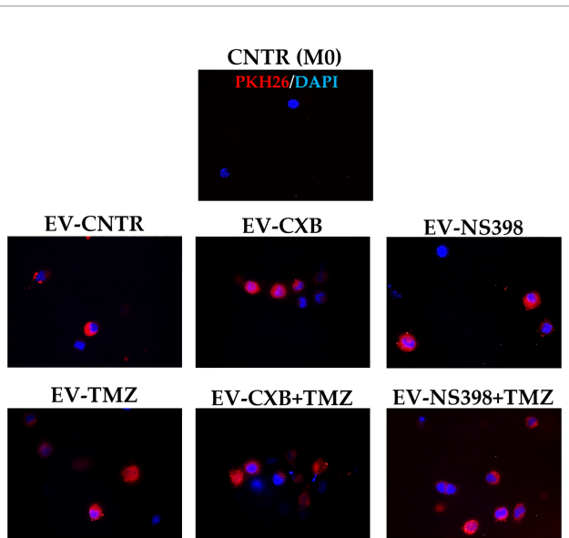
FIGURE 5 | Macrophage U937 intracellular uptake of EV derived from control (CNTR) and CXB-, NS398-, TMZ-, drugs combination-treated T98G assessed by PKH26 staining. PKH26-labeled EV-COX-2 (red) were incubated at 30 \mu\text{g}/\text{ml} with U937 cells for 18 h. The nuclei of U937 were counterstained with DAPI (blue). CNTR (M0) = U937 cells not exposed to EV. Representative immunofluorescence images are from one out of three independent experiments. All images were acquired at 100 \times magnification.
