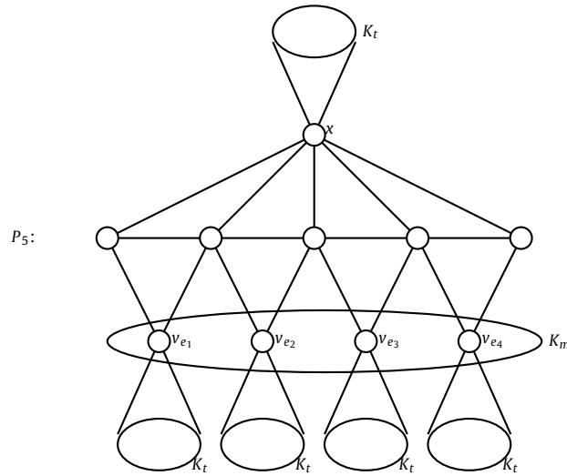
Fig. 1. Construction of the graph G' from G = P_5 .
