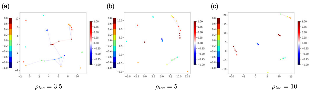
Figure 9. Network fragmentation and opinion homogeneity. Network while increasing the radius of interaction and keeping the same attitude function, i.e. Blue : r_f = 0.15 , r_a = 0.20 , r_r = 0.30 , r_l = 0.40 .
