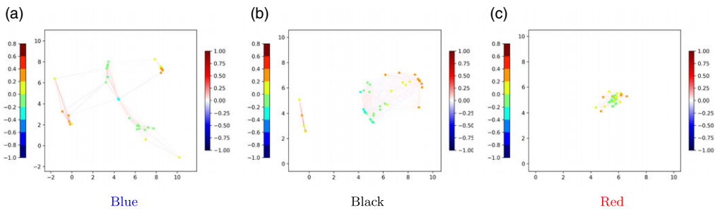
Figure 7. Final network distribution. The olive function has not been plotted because it describes an extreme behaviour, all the agents collapse very fast into a unique point.
