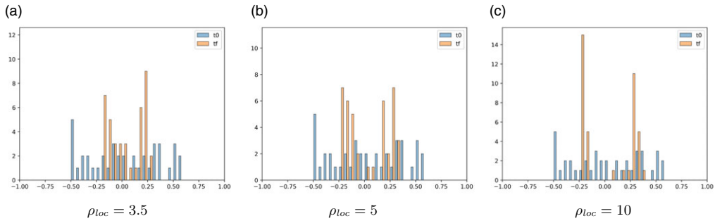
Figure 6. Initial and final mean opinions distribution. In this figure, in blue the distribution of the mean opinions at time t = 0 , and in orange the mean opinions' distribution at final time (which corresponds to the time showing a quasi-stable status of the simulation result). We observe that the final distribution tends to have two peaks, which means that the opinions of the population are more and more split into two opinion groups. However, they are also more close to the centre. This means that we observe a sort of fragmentation and radicalisation, but there is no polarisation.
