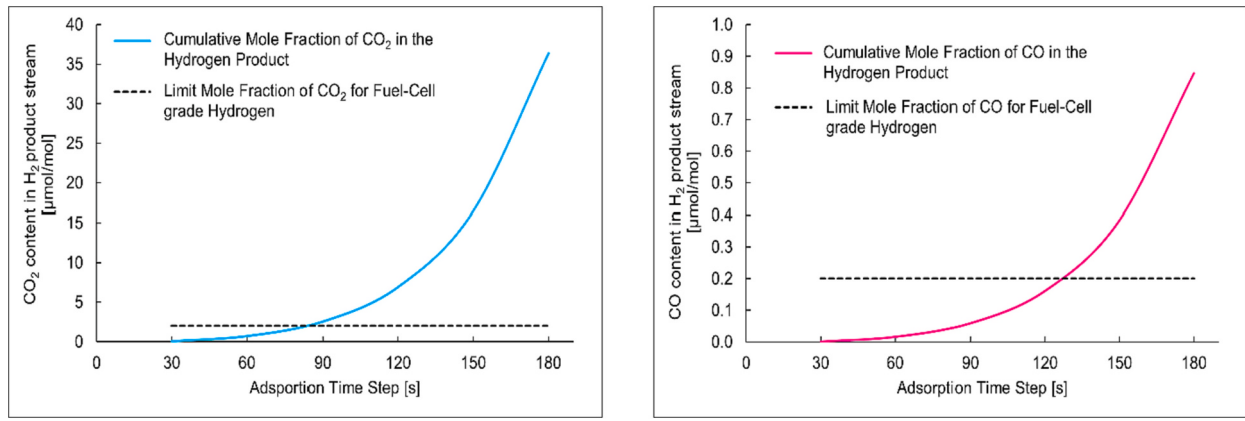
Fig. 4. a) \text{CO}_2 content in the outlet hydrogen product stream as a function of adsorption time step, along with the 2 \mu\text{mol/mol} limit required for fuel-cell-grade hydrogen (dashed black line); b) CO content in the outlet hydrogen product stream as a function of adsorption time step, along with the 0.2 \mu\text{mol/mol} limit required for fuel-cell-grade hydrogen (dashed black line).
