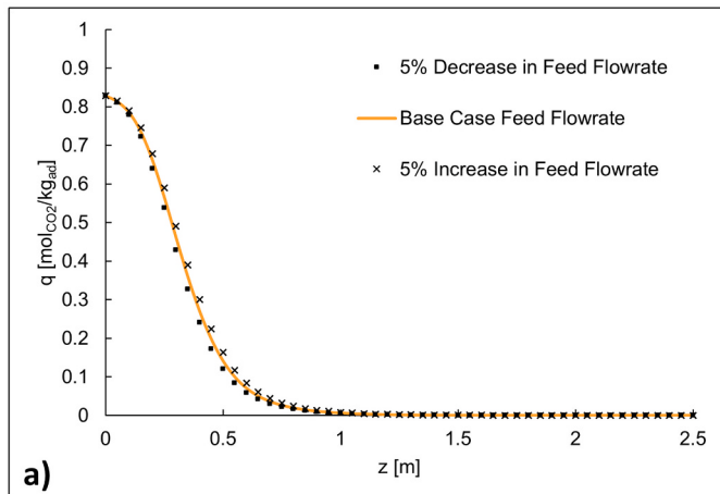
Fig. 6. a) \text{CO}_2 adsorbed on the sorbent as a function of the column length at the end of the adsorption step at various feed flowrate; b) \text{CO}_2 adsorbed on the sorbent as a function of the column length at the end of the adsorption step with increased \text{CO}_2 content in the feed. Adsorption time of 60 s. Total reactor length: 2.5 m.
