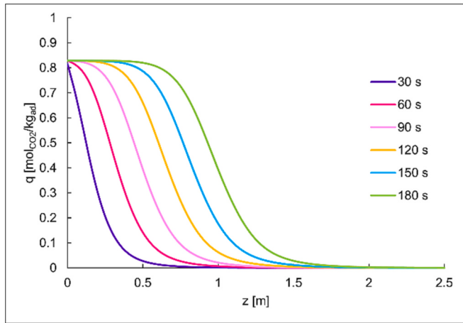
Fig. 5. \text{CO}_2 adsorbed on the sorbent as a function of the column length at various adsorption time step. Total reactor length: 2.5 m.
