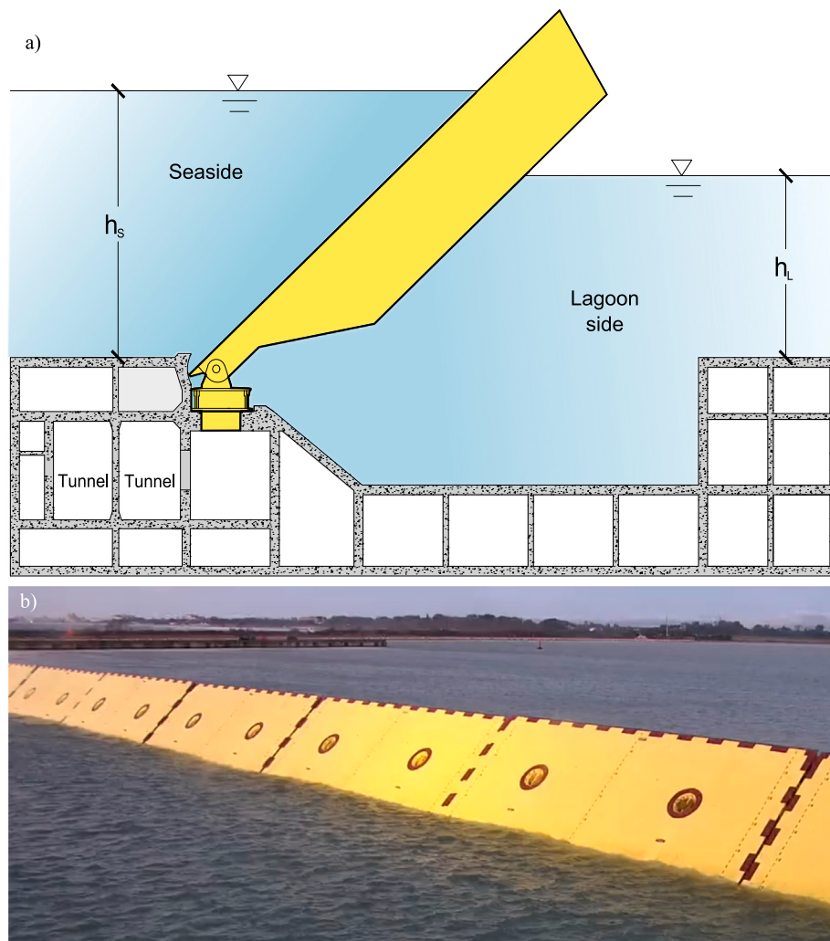
Fig. 2. Panel (a). Scheme of a single gate hinged at the cellular caisson that lies on the inlet bottom. h_s and h_L are the sea and lagoon levels, respectively. Panel (b). The MoSE barrier of Lido San Nicolò during the operation phase. The picture is taken from the seaside towards the lagoon side. Photo courtesy of Consorzio Venezia Nuova.
