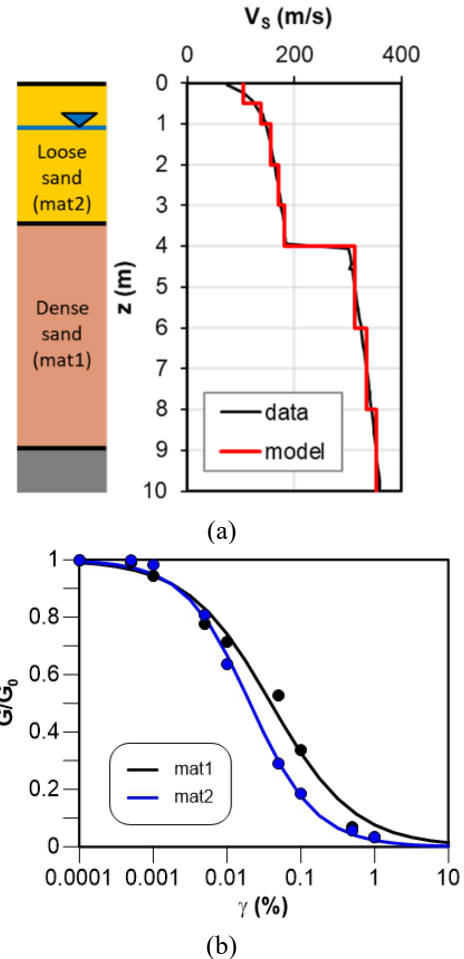
Figure 5. (a) Ideal soil column and (b) normalized shear modulus vs. shear strain for mat1 and mat2 and analytical curves adopted in the analyses (MKZ model)
