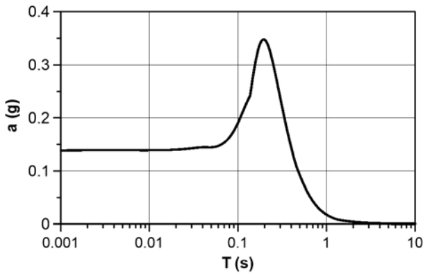
Figure 7. Input motion.
