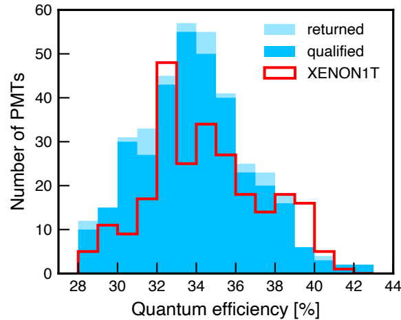
Figure 2. Quantum efficiency (QE) distribution for the full set of the 368 tested PMTs, measured for 175 nm photons at 25 °C. The darker shaded blue distribution corresponds to the PMTs that passed all tests described in this report and thus qualified for use in XENONnT. The lighter shaded blue distribution stacked on top represents PMTs that failed any of the tests and were returned to the manufacturer for replacement. The QE distribution of the 248 PMTs used in the XENON1T detector are shown in red [10]. All values are provided by Hamamatsu.
