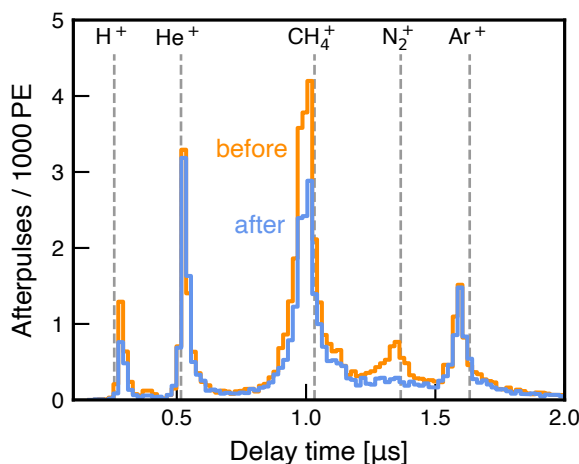
Figure 11. Comparison of two afterpulse timing spectra of the same PMT, acquired at room temperature before (orange) and after (blue) two cooling cycles in gaseous argon. The afterpulse lines corresponding to hydrogen H^+ , methane CH_4^+ and nitrogen N_2^+ are reduced after the exposure to cryogenic temperatures.
