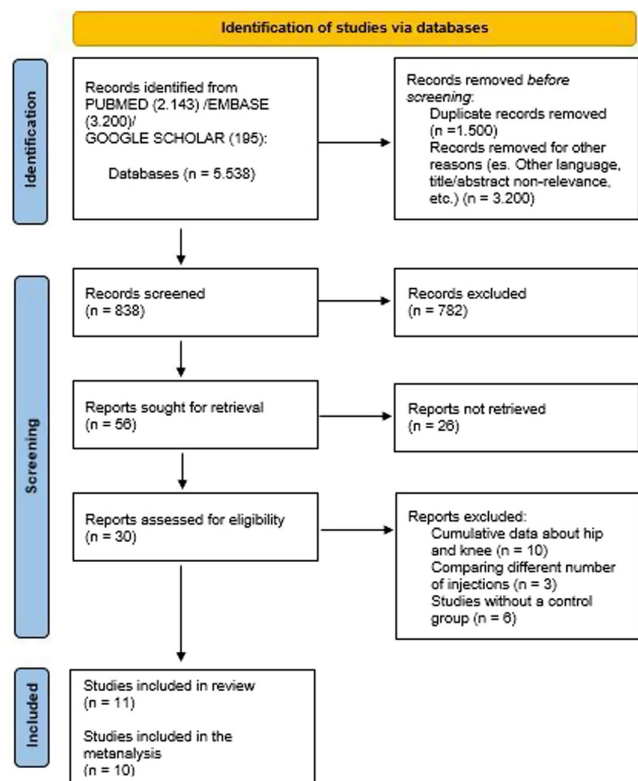
Figure 1 Study flowchart.
