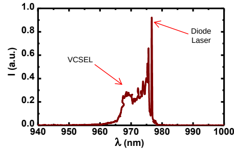
Fig. 6. Spectrum of VCSEL emission (below threshold, Fig. 3(e)) with superimposed spectrum of injected beams ( \text{FWHM} \approx 0.43 nm) from the diode laser (LD) in experimental conditions.
