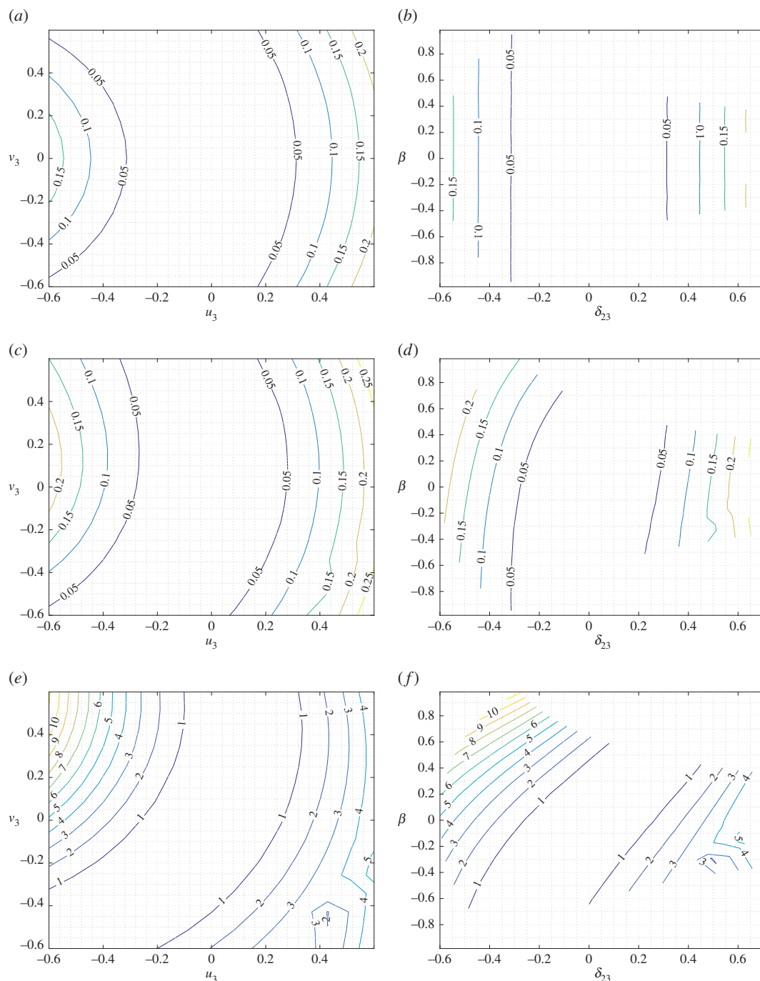
Figure 7. King post truss: level sets for the strain energy W for \delta_{12} = 0 varying a in the plane u_3 - v_3 ( a,c,e ) and in the plane \delta_{23} - \beta ( b,d,f ). ( a,b ) a = 0.01 , ( c,d ) a = 1 and ( e,f ) a = 100 .
