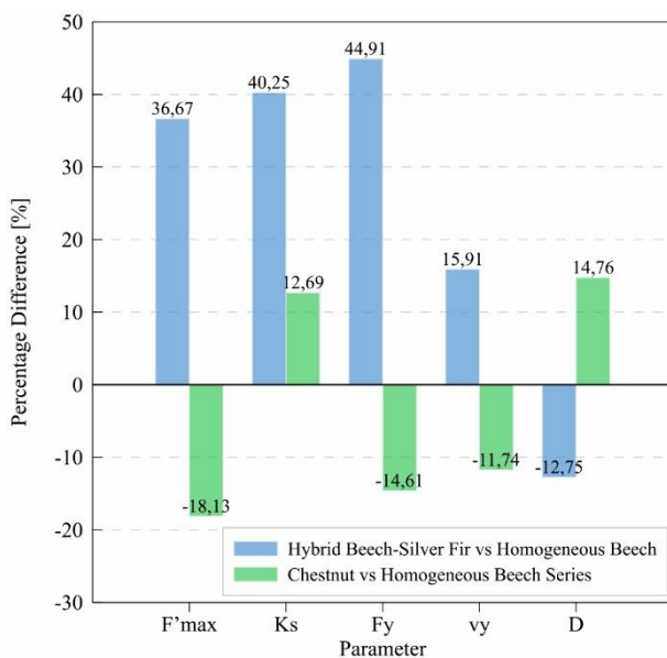
Figure 4. Comparison of experimental evidence among the series
