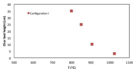
Figure 2 Temperature in the fixed bed
