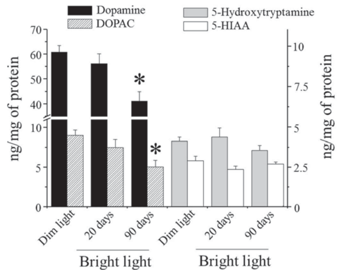
Figure 4 | Levels of dopamine, DOPAC, 5-hydroxytryptamine and 5-HIAA in rats raised in dim light–dark cycle and rats raised for 20 days or 3 months under bright light. The scale indicating dopamine and DOPAC levels is on the left y-axis while 5-hydroxytryptamine and 5-HIAA levels refer to the right y-axis. *Significantly different from animals raised in dim light – dark cycle (dopamine: F_{10,8,8} = 9.01461 , p = 0.00129 ; DOPAC: F_{10,8,8} = 6.42800 , p = 0.00606 , using one way ANOVA plus Scheffe's F test).
