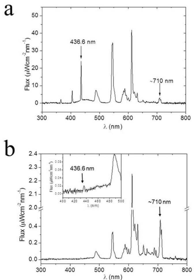
Figure 1 | Light spectrum of the fluorescent lamp used to illuminate the animals. (a) Light spectrum measured in the cages where the animals were housed and (b) light spectrum of the same lamp measured from the inside of the rat scalp and skull. The inset in panel (b) is a magnification of the spectrum between 400 and 500 nm to show the pick at 436.6 nm.
