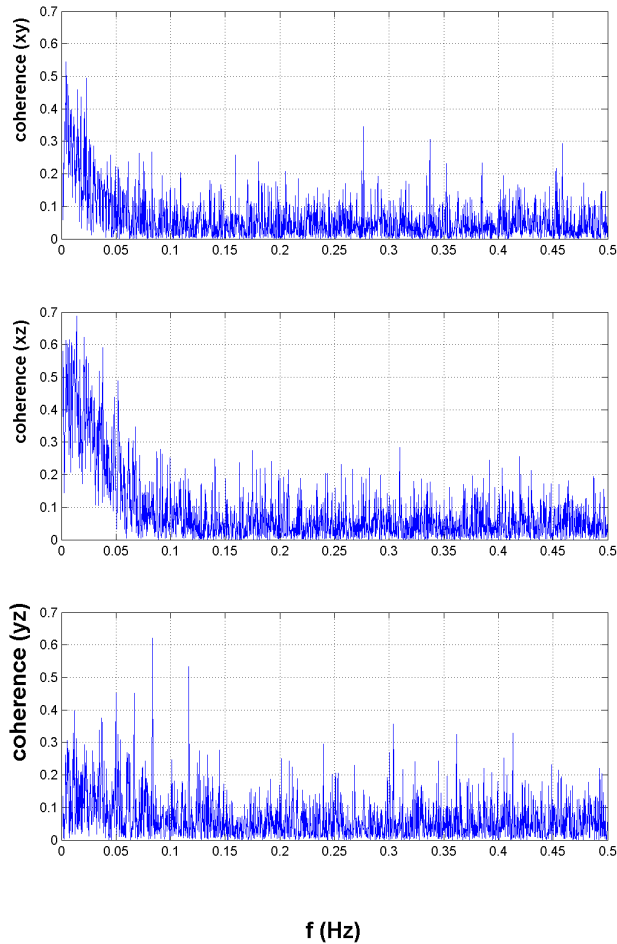
Figure 9. Coherence analysis between the three components of geomagnetic field.
