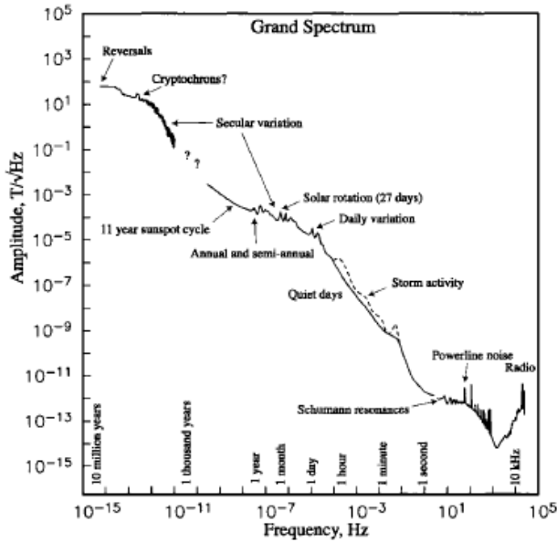
Figure 1. Power spectra of the variations of the geomagnetic field (adopted from Constable and Constable [2004]).
