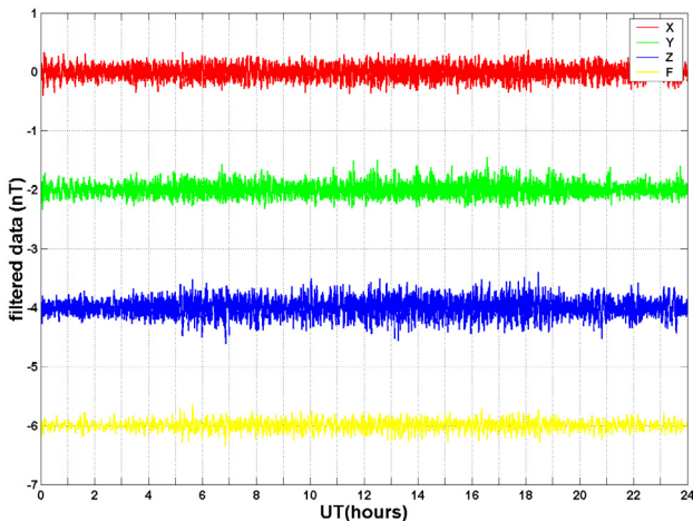
Figure 5. Example of geomagnetic filtered data (components X, Y, Z and total intensity F) relative to a selected day with local K index approximately zero.
