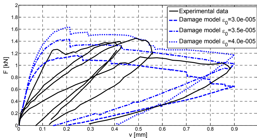
Figure 4: Response of the masonry arch: comparison between the experimental result data and numerical results obtained for different values of the \epsilon_0 .
