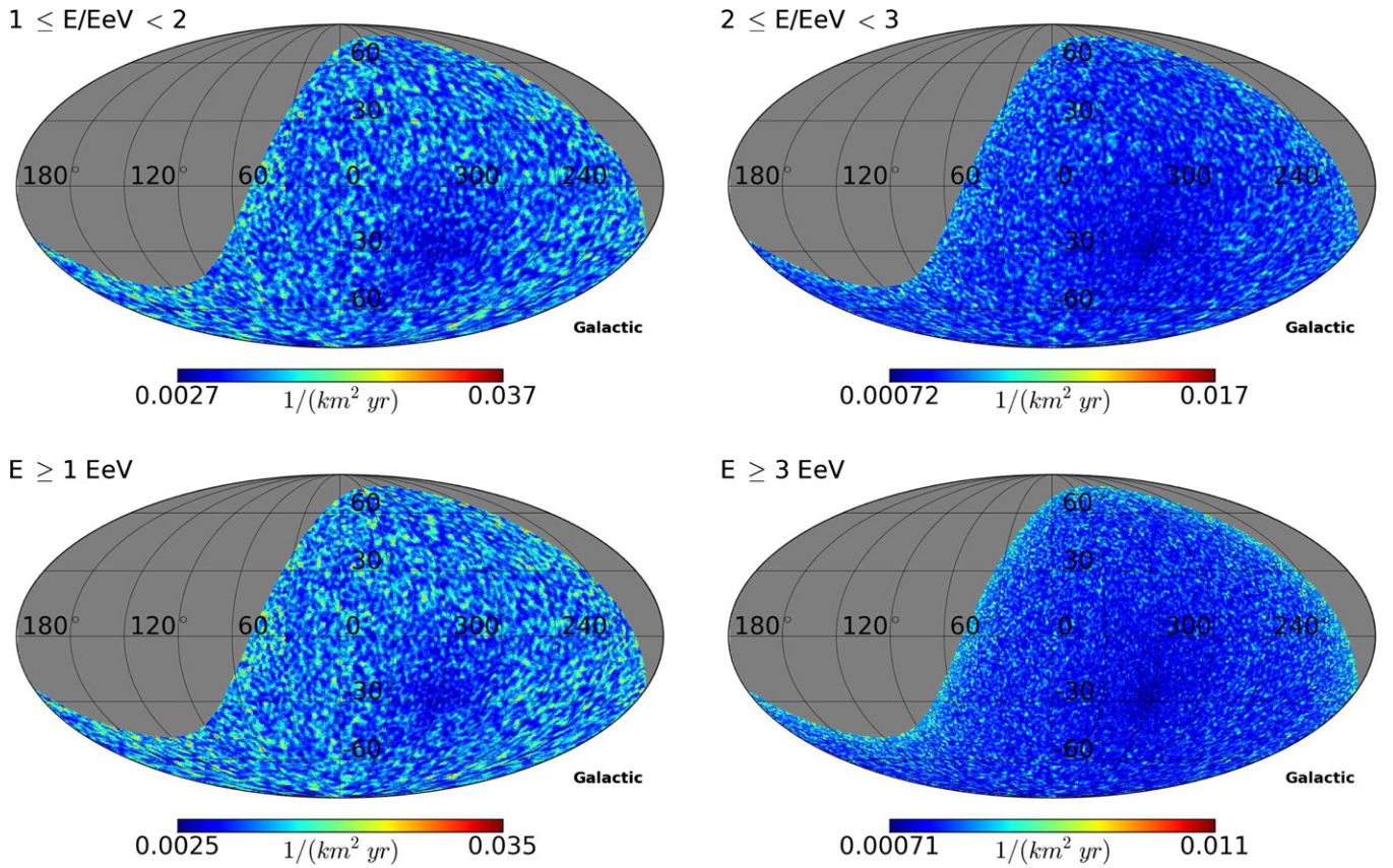
Figure 4. Celestial maps of the flux upper limit (particles/km 2 yr) in Galactic coordinates. (A color version of this figure is available in the online journal.)
