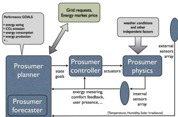
Fig.2: General scheme of the prosumer node reference model.
