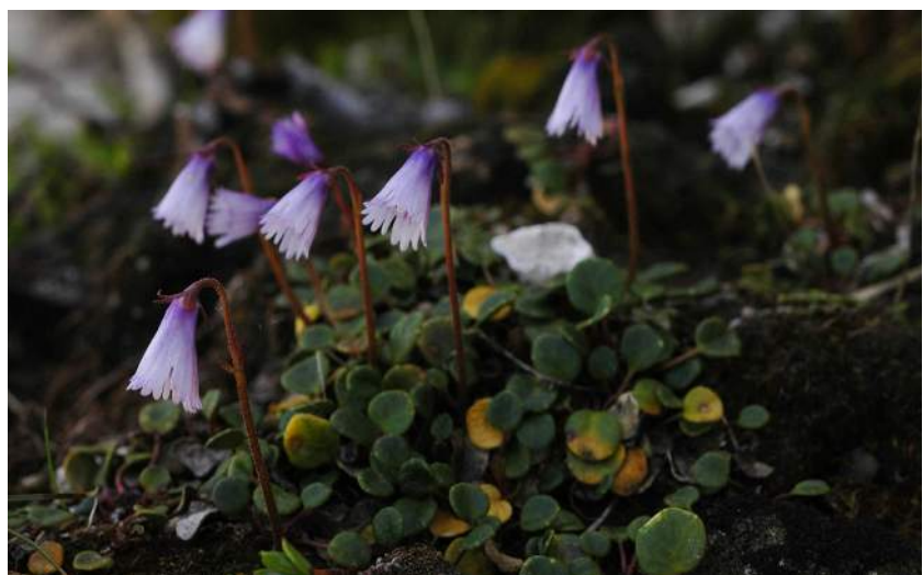
FIGURE 2. Soldanella minima subsp. samnitica , endemic species of Majella
