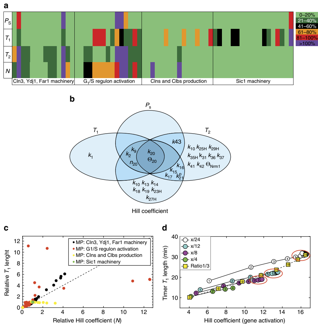
Figure 5 | Parameter-sensitivity analysis. (a) Heat map describing the effect of parameter variation on the outputs of the G 1 /S transition model. (b) Venn chart summarizing the parameters whose variation affects one or more outputs of the G 1 /S transition model. (c,d) Correlation analysis of the changes in T_1 length as a function of the changes in the Hill coefficient N . Each point in c refers to a single-cell simulation in which one model parameter—colour-coded by functional class—was altered. The x and y axes are the relative output values, with the value of the standard parameter set to 1. The black dotted line represents the expected output for a 1-to-1 correlation. Each point in d refers to a single-cell simulation in which different Whi5 phosphorylation settings were considered. Coloured circles refer to simulation sets with a fixed total number of phosphorylation sites and a variable number of functional sites (indicated within the circle itself). Yellow boxes refer to simulation with fixed (1/3) ratio of functional/total phosphorylation sites. The total number of sites is indicated within the square.
