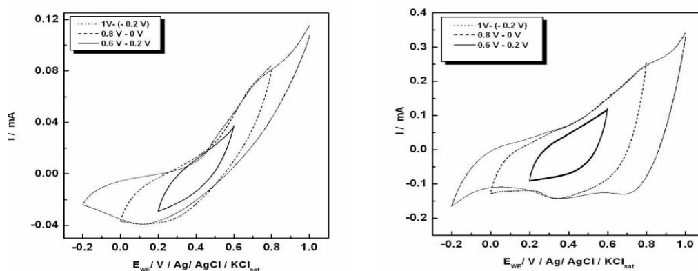
Fig. 3 Cyclic voltammograms of S1 and S2 over different potential ranges, in 1\text{M Na}_2\text{SO}_4 , 5\text{mV/s}
