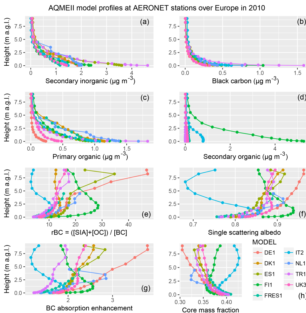
Figure 2. Average model profiles sampled at locations and timings of AERONET observations available for the year 2010 over Europe. Panels (a)–(d) show the simulated aerosol species concentrations included in the subsequent optical calculations. The ratio of total concentration of secondary inorganic aerosol (SIA) and organic carbon (OC, primary plus secondary) to black carbon (BC) also qualitatively illustrates the air mass chemical aging (larger for more aged aerosol). The single scattering albedo is that calculated using external mixing assumption (simulation EXT in Table 4). BC absorption enhancement is the ratio of absorption optical depths of simulation CSBC (core-shell internal mixing) to EXT. The core mass fraction is that calculated in the CSBC simulation.
