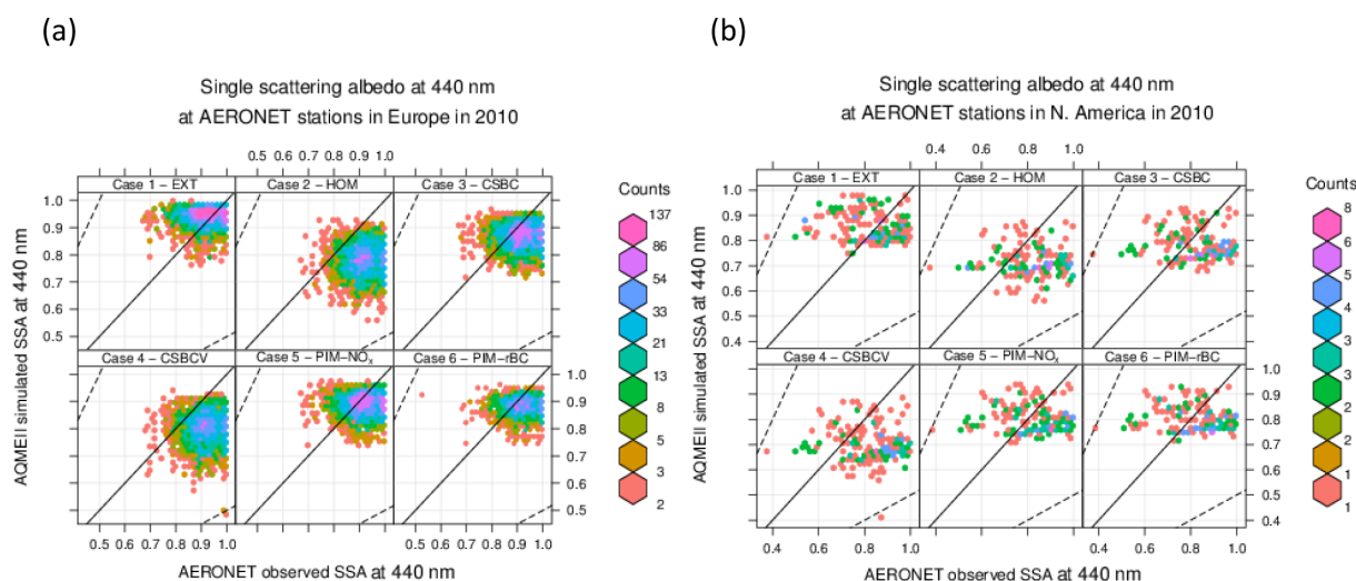
Figure 5. Comparison of FlexAOD modelled and observed single scattering albedo at 440 nm ( \omega_{0,440} ) for 2010 at AERONET stations over (a) Europe and (b) North America, only for scenes classified “BC” or “BC + BrC”-dominated, and having a modelled aerosol volume concentration and effective radius within a factor of 2 of observations. Simulation labels are defined in Table 4.
