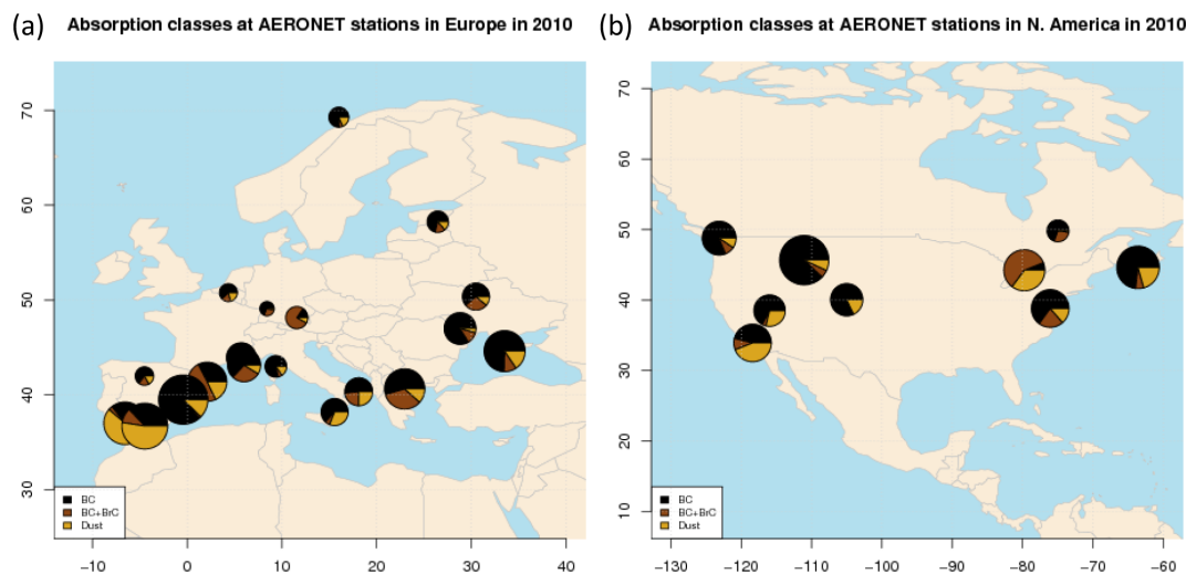
Figure 1. Location of AERONET sunphotometer stations selected over (a) Europe and (b) North America. We use Level 2.0 inversion products for the year 2010, filled with Level 1.5 for scenes where absorption data (spectral single scattering albedo and absorption aerosol optical depth) were discarded in Level 2.0. The pie charts display the relative abundance of scenes classified as dominated by “dust” (dark yellow), “black carbon” (black), or “black carbon + brown carbon” (brown). The size of the pies is proportional to the total number of observations.
