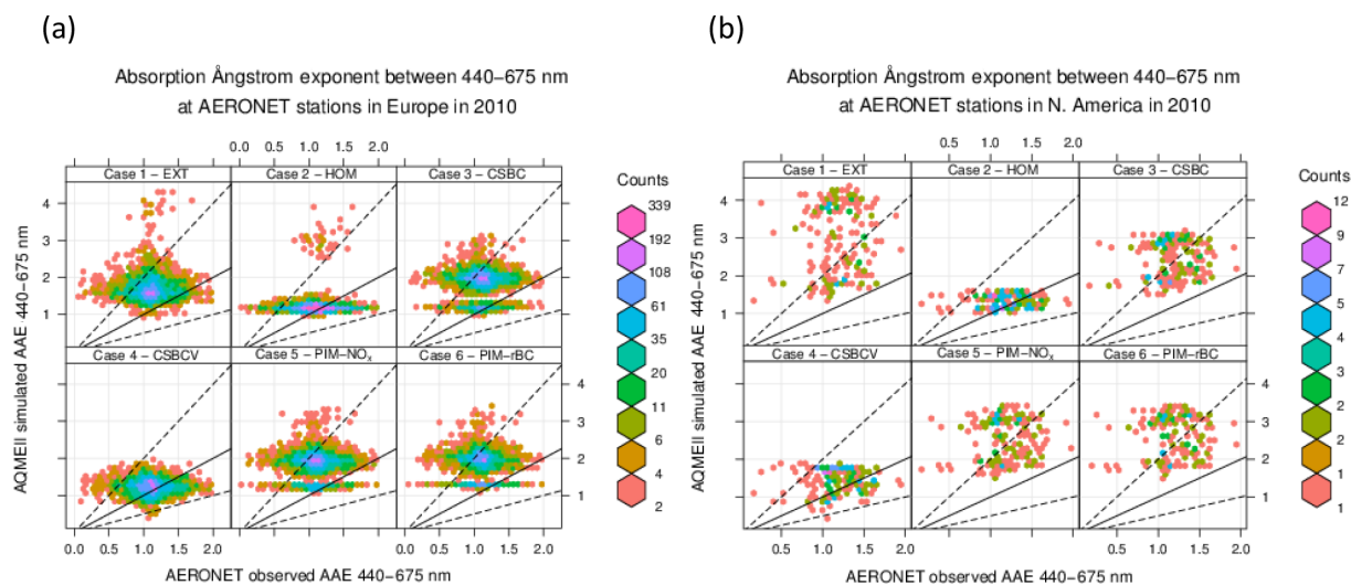
Figure 8. Same as Fig. 5 but for the absorption Ångström exponent between 440 and 675 nm ( AAE_{675}^{440} ).
