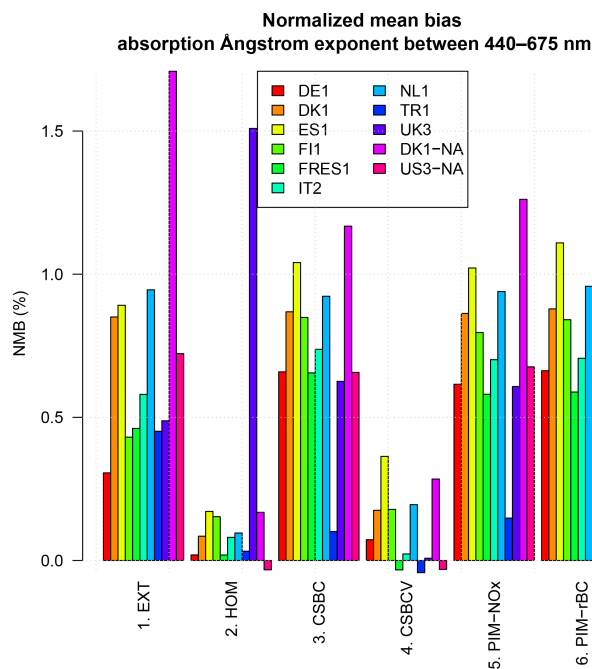
Figure 9. Same as Fig. 6 but for the absorption Ångström exponent between 440 and 675 nm ( AAE_{675}^{440} ).
