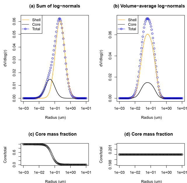
Figure 4. Illustration of the different combination of size distributions tested in sensitivity simulations CSBC (a, c) and CSBCV (b, d). The size distributions of each species can be kept unchanged and summed in each size bin with the others (CSBC, a, c), or a single volume-average size distribution for all species can be computed (CSBCV, b, d). On (c) and (d) the resulting core mass fractions are shown as a function of particle radius. A lower core mass fraction is typically associated with higher core absorption enhancement.
