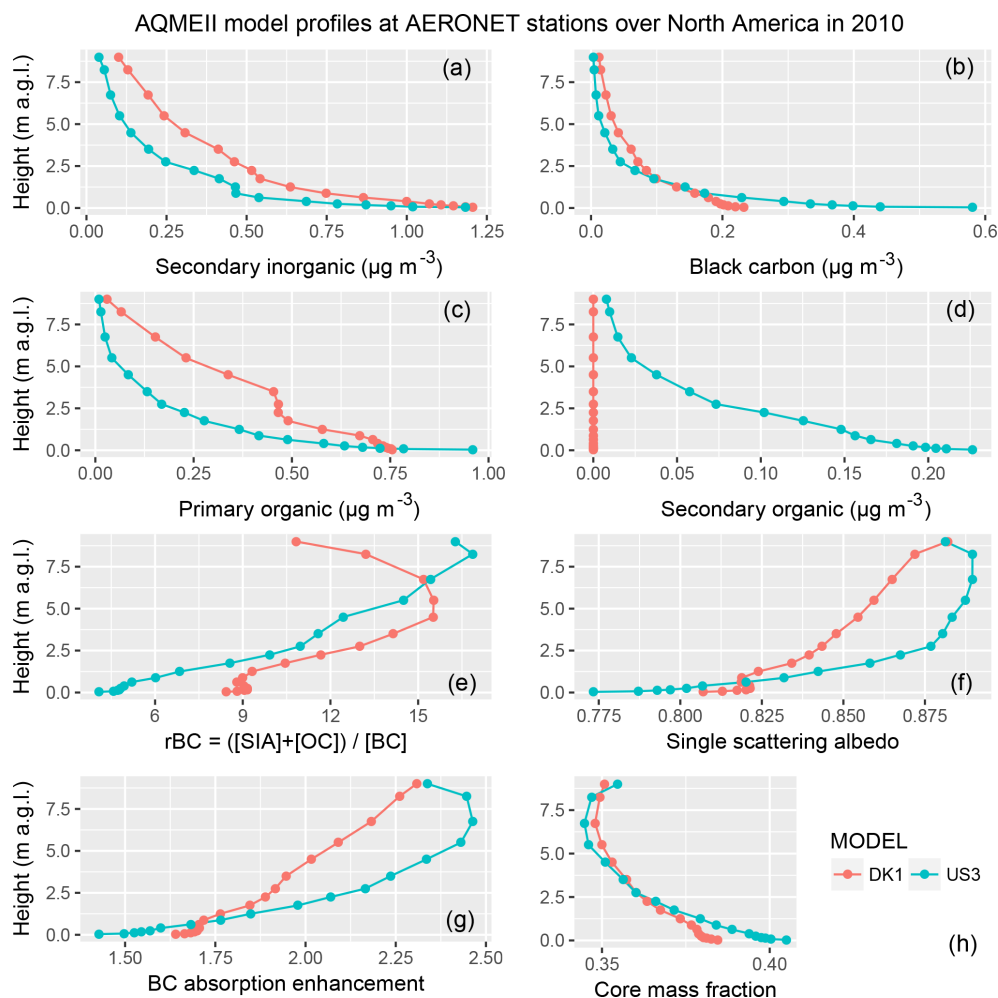
Figure 3. Same as Fig. 2 but for North America.
