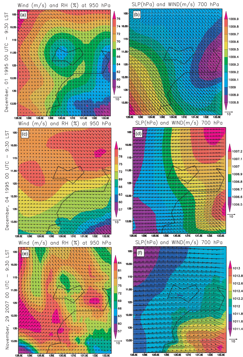
Figure 1. ECMWF analysis over the Tiwi Islands at 00:00 UTC for D1, D4 and N29. Panels (a, c, e) report surface wind and relative humidity at 950 hPa; panels (b, d, f) report sea level pressure in filled contours and wind flow vectors at 700 hPa.
