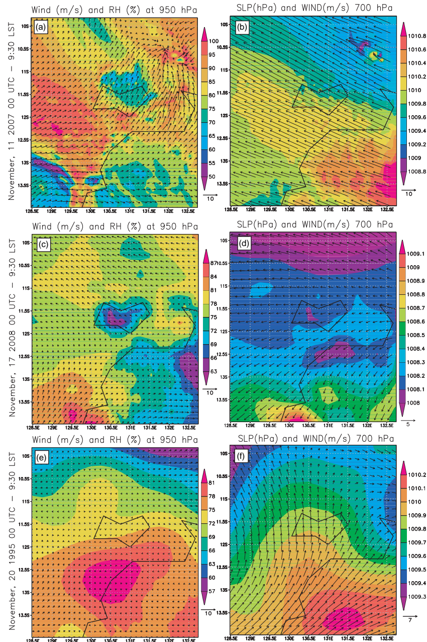
Figure 2. ECMWF analysis over the Tiwi Islands at 00:00 UTC for N11, N17 and N20. Panels (a, c, e) report surface wind and relative humidity at 950 hPa; panels (b, d, f) report sea level pressure in filled contours and wind flow vectors at 700 hPa.
