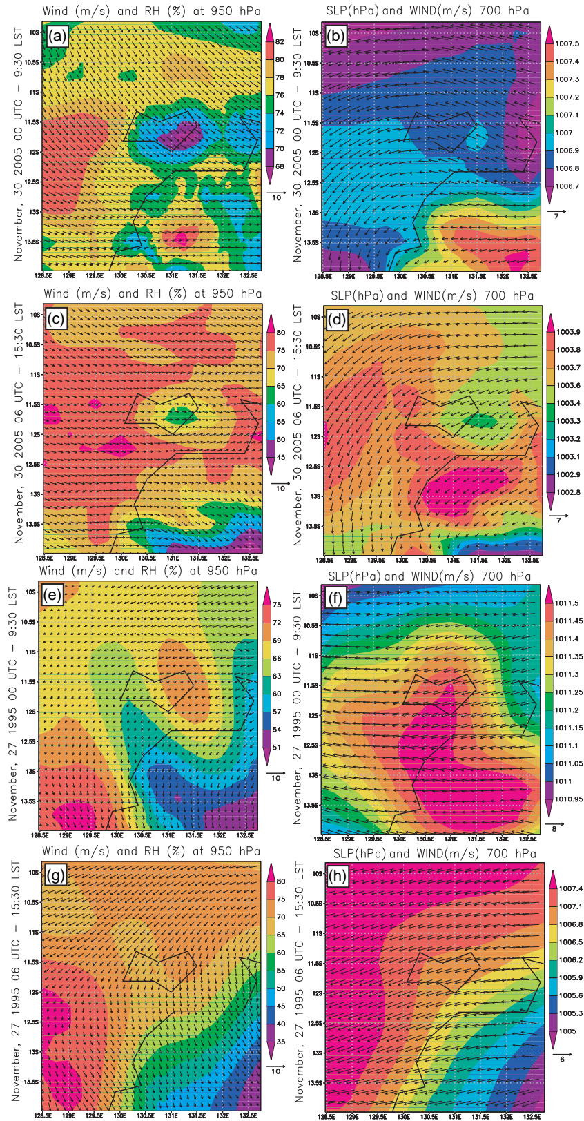
Figure 4. ECMWF analysis over the Tiwi Islands for N30 and N27 at 00:00 UTC for the first cell and at 06:00 UTC for the second one. Panels (a, c, e, g) report surface wind and relative humidity at 950 hPa; panels (b, d, f, h) report sea level pressure in filled contours and wind flow vectors at 700 hPa.
