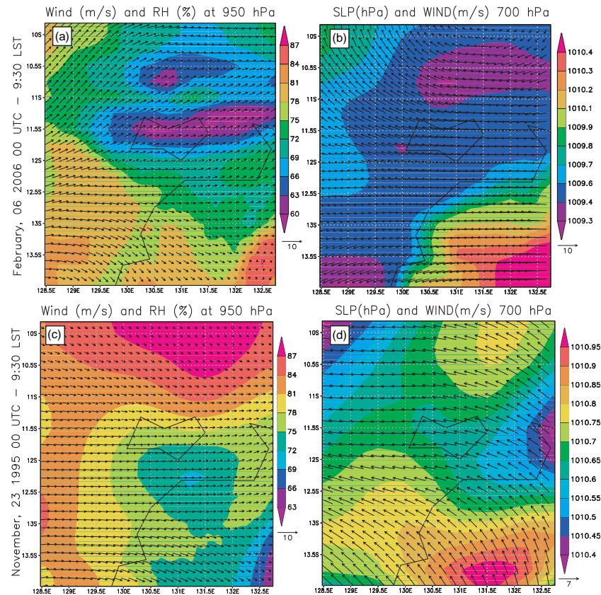
Figure 3. ECMWF analysis over the Tiwi Islands at 00:00 UTC for F6 and N23. Panels (a, c) report surface wind and relative humidity at 950 hPa; panels (b, d) report sea level pressure in filled contours and wind flow vectors at 700 hPa.
