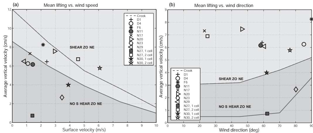
Figure 8. Crook's test: panels (a) and (b) show vertical velocity at 500 m extracted 3 h before the maximum development versus surface wind speed (a) and surface wind direction (b), both extracted at the start time. The figure reports two different regimes with a sheared (light gray, dashed line) and unsheared flow (dark gray, solid line) as studied by Crook.
