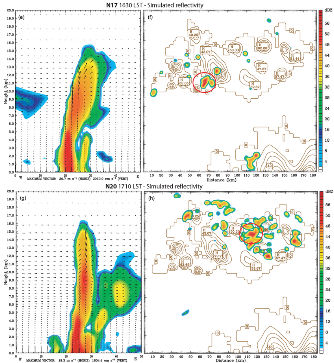
Figure 6. Sections at the maximum development of the Hector events N23, N11, N17 and N20. (a, c, e) Simulated vertical radar reflectivity (dBZ; filled color) and vertical wind, the section is taken longitudinally along the red circle reported in the right panel. (b, d, f) Horizontal radar reflectivity (dBZ; filled color) and topography (brown).
