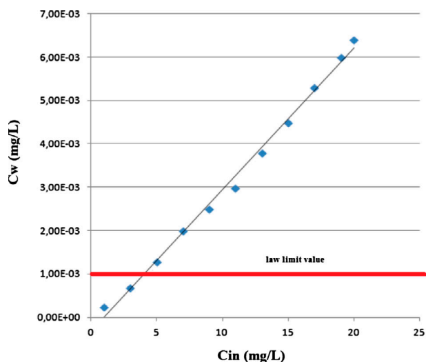
Fig. 6. Benzene concentration in the water phase in the outlet reactor stream for different initial benzene concentration in the reactor. Comparison with law limit concentration (0.001 mg/L) of benzene for agricultural water purpose.
