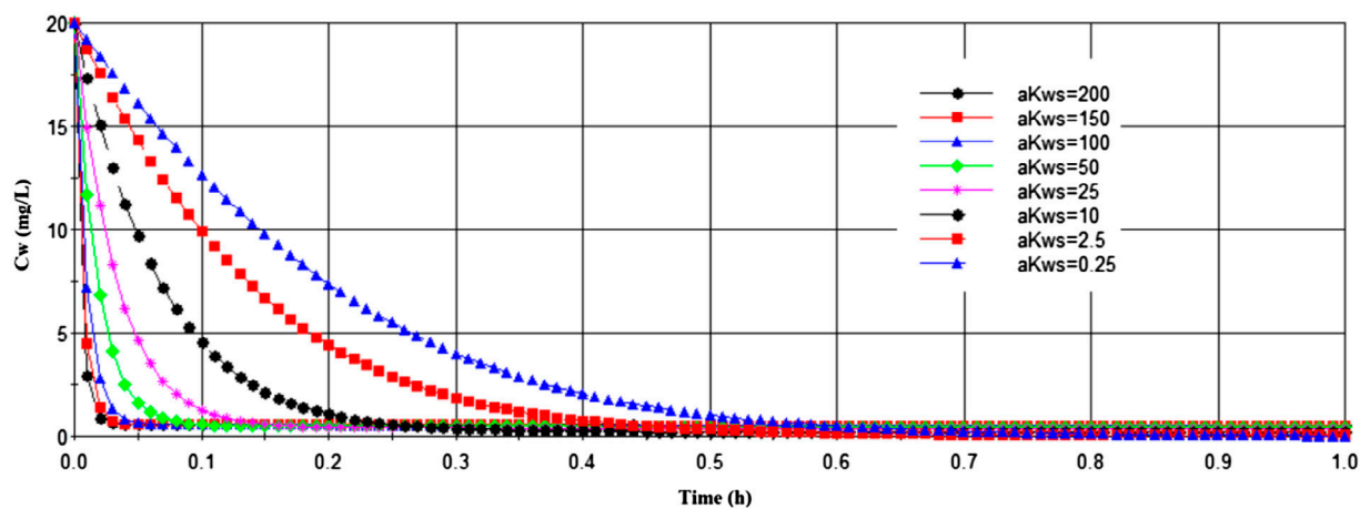
Fig. 5. Influence of xenobiotic mass transfer coefficient between organic and water phases on reactor removal performance.
