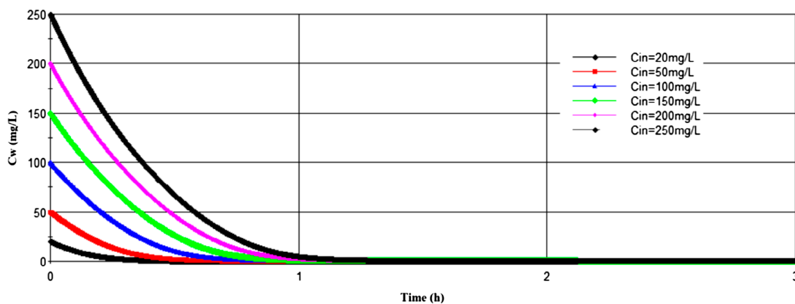
Fig. 3. Influence of initial xenobiotic concentration in the water phase ( C_{in} ) on reactor removal performance.
