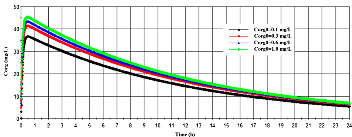
Fig. 4. Influence of initial xenobiotic concentration in the organic phase ( C_{org0} ) on reactor removal performance.
