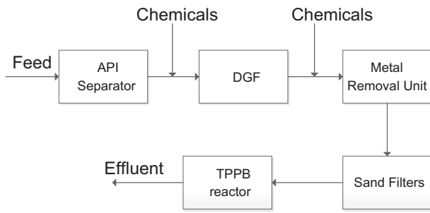
Fig. 1. Block scheme of the PW treatment.
