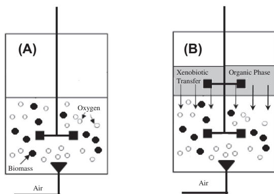
Fig. 2. Schematic representation of the SBR (A) and TPPB (B) reactors during the reaction phase.
