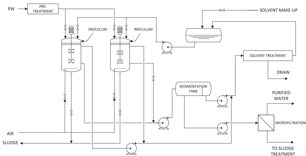
Fig. 7. PW treatment: process scheme.
