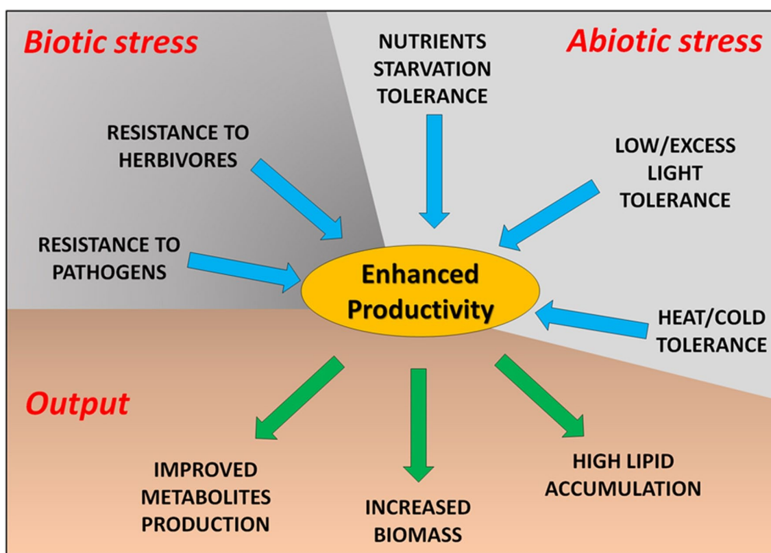
Fig. 3 Schematic depiction of the major desirable traits to be either implemented or improved, toward higher productivity of microalgae in mass culture
