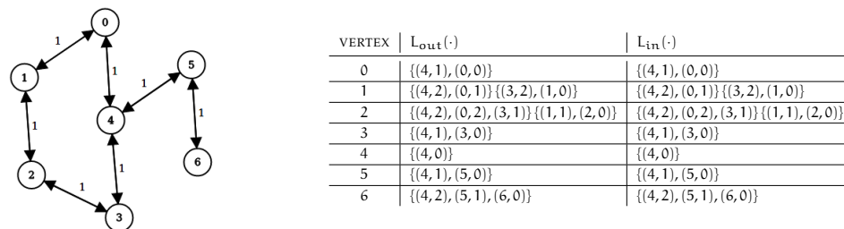
Figure 4. Consider again the graph of Figure 1 and a corresponding 2-HOP-COVER labeling. Assume arc (4, 0) is removed. We have that vertex 3 is in F_G^L(0, 1) and vertex 0 is in B_G^L(0, 1) . However, there is no outdated label entry in L_{out}(3) but the decremental operation on arc (4, 0) causes the cover property to be broken for pair (3, 0) .
