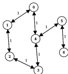
Figure 1. A sample graph and a corresponding 2-HOP-COVER labeling is shown. Vertex ordering is {4, 0, 3, 1, 2, 5, 6}.
