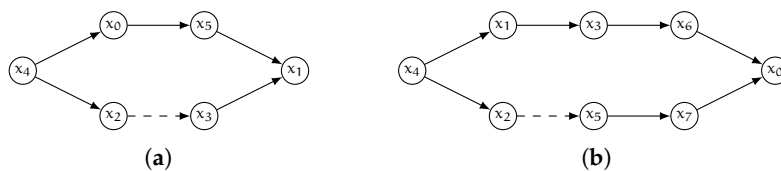
Figure 5. (a): an example of the contradiction reached in the proof of Property 3. Suppose vertex ordering is \{x_0, x_1, x_2, \dots, x_5\} and all arcs weight 1 for the sake of the example. Therefore, in any minimal well-ordered 2-HOP-COVER labeling entry (x_1, \delta_{x_4x_1}) cannot belong to L_{out}(x_4) . This allows Algorithm CLEAN to avoid removing correct entries. (b): a case where a correct entry is preserved by Algorithm CLEAN. Suppose the vertex ordering is \{x_0, x_1, x_2, \dots, x_7\} and all arcs weight 1 for the sake of the example. Therefore in any minimal well-ordered 2-HOP-COVER labeling, L_{out}(x_4) will contain (x_0, \delta_{x_4x_0}) with \delta_{x_4x_0} = d(x_4, x_0) = 4 . Clearly, also L_{out}(x_1) and L_{out}(x_2) will contain, similarly, entries (x_0, 3) and (x_0, 3) , respectively. If arc (x_2, x_5) undergoes some decremental update, the (correct) entry in L_{out}(x_4) is not removed thanks to the presence of the alternative shortest path through x_1 with the same weight as that through x_2 .
