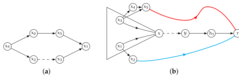
Figure 6. (a): an example of the contradiction reached in the proof of Lemma 3. Suppose vertex ordering is \{x_0, x_1, x_2, \dots, x_5\} and all arcs weight 1. Therefore, in any minimal well-ordered 2-HOP-COVER labeling, entry (x_1, \delta_{x_4 x_1}) cannot belong to L_{out}(x_4) , due to the pruning test succeeding because of x_0 . Also, in this case no correct entry is removed by Algorithm CLEAN. (b): restore phase for vertex r .
