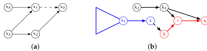
Figure 3. (a): assume all arcs in this example have unitary weight and the vertex ordering is \{x_0, x_1, \dots, x_4\} . Both x_4 and x_3 are in F_G^L(x_1, x_0) since the hub vertex for pairs x_4, x_0 and x_3, x_0 , in the labeling L induced by the above ordering, is vertex x_0 . However, if arc (x_1, x_0) is removed then d_G(x_4, x_0) changes while d_G(x_3, x_0) does not, since x_3 has two shortest paths of the same weight to x_0 . (b): In the toy graph G shown here the only shortest path from x to h passes through arc (x, y) . Therefore, if (x, y) undergoes a decremental update, we have that x, x_1 , and all vertices that are connected to x_1 , are in the forward cover graph (in blue). Symmetrically, r and h are in the backward cover graph (in red) while k_1 and k_2 are in neither of the two cover graphs.
