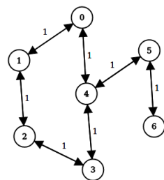
Figure 2. Consider the graph of Figure 1 (left) and the corresponding labeling (right). Assume arc (4, 0) is removed. If Algorithm BIDIR-2HC is executed, vertices 3, 5, 6 have their label sets scanned twice, once during the detection of affected vertices and once during the removal phase, since hub vertex for pairs (3, 0) , (5, 0) and (6, 0) is vertex 4. However, no label entry is removed from L_{in}(3) nor from L_{out}(3) (the same hold for label sets of L_{in}(5) , L_{out}(5) , L_{in}(3) , L_{out}(3) ). Our algorithm instead scans these label sets only once.
