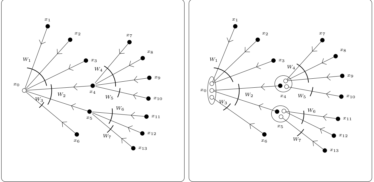
FIGURE 3. The weight (4.1) of an enriched digraph is a product of contributions of building blocks. The left panel represents an enriched digraph with weight
