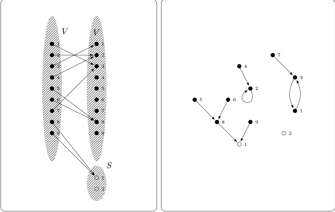
FIGURE 1. Relation between partial endofunction and the associated functional digraph. On the left hand side an endofunction in the usual representation of a functions is given. On the right hand side the functional digraph associated to the endofunction in the left box is drawn.
