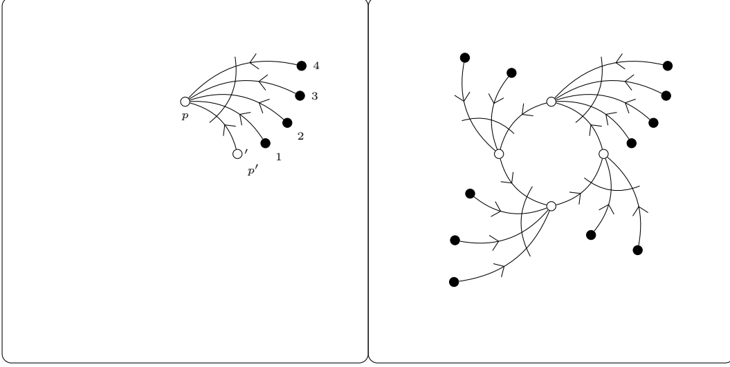
FIGURE 4. The left panel shows a spike with k = 4 . The right panel shows a crown, where the set of white vertices the base B and V (as in Definition 4.7) is the set of all white and black vertices. The partitions P_r are symbolized by the small curved lines crossing the edges.
