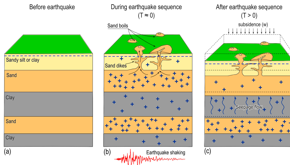
Figure 8. Conceptual scheme of the liquefaction effects and post-liquefaction subsidence developed in the study area. (a) Typical stratigraphic column of the investigated area before the earthquake sequence as in Figure 2. (b) Effect of the earthquake shaking, with increased pore pressures (the blue ‘plus’ symbols) and the formation of sand boils at the surface, with water leaks from cracks. (c) Post-seismic upward seepage flow and excess pore pressure dissipation after the earthquake sequence, with an accumulation of ground subsidence.
