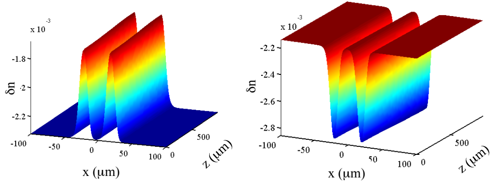
Fig. 2. Numerically calculated refractive index \delta n(x, z) in the PRC for the opposite values V_e = 37.5 V (left) and V_e = -37.5 V (right). For negative values of V_e we expect that the injected radiation propagates confined along the PRC center.
