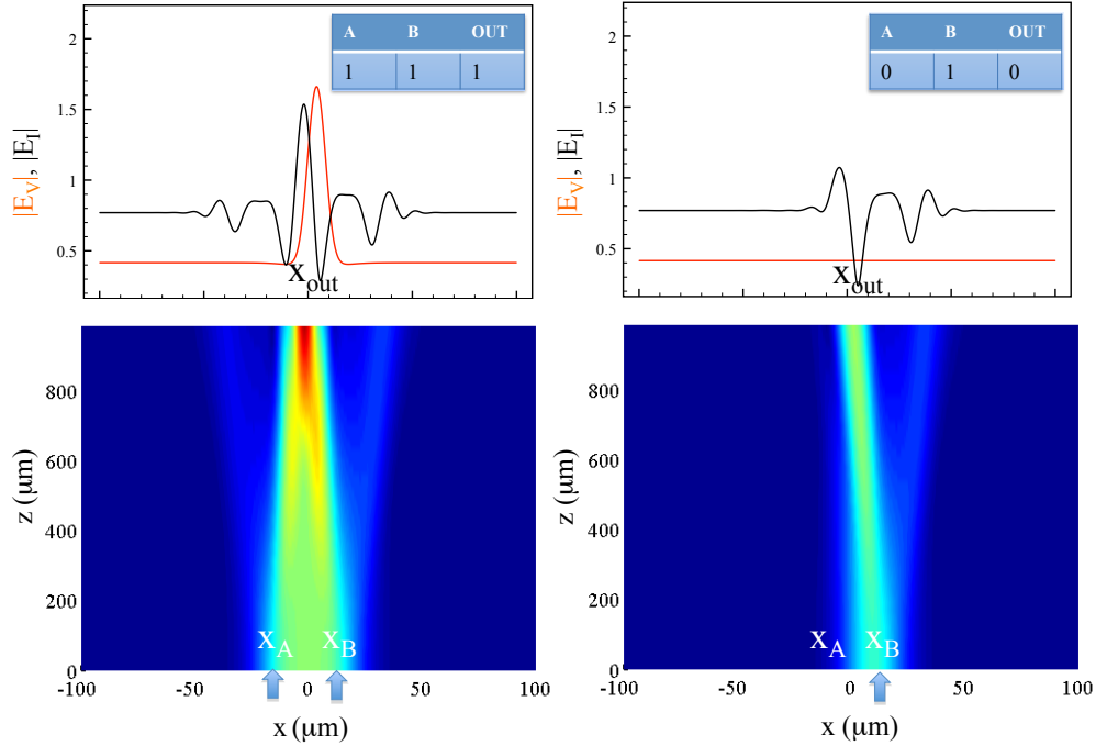
Fig. 3. Logic AND for V_e = -37.5 V. In the bottom panels it is shown the field amplitude in the PRC (in the color scale the dark red corresponds to the maximum amplitude). The black and red lines in the upper panel represent the injected field amplitude and the field amplitude at steady state in the VCSEL respectively. A CS is switched on and persists in X_{Out} if and only if two input Gaussian beams are launched in X_A and X_B . As indicated by the arrows, (left) and (right) refer to the input (1, 1) and (0, 1) respectively.
