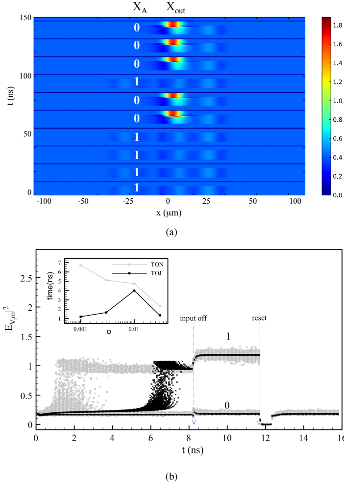
Fig. 6. Eye diagram for a NOT A gate. We plot the electric field intensity in the VCSEL averaged over an interval of \simeq 20 \mu\text{m} centered at X = 0 \mu\text{m} ( |E_{V,m}|^2 ) for 300 operation cycles as described in the text. (a) Temporal variation of the electric field amplitude in the VCSEL during a sequence of 10 operation cycles associated with 10 random values of the input A. (b) Eye diagram for the NOT A logic gate in presence of noise with amplitude \sigma = 0.001 (black symbols) and \sigma = 0.03 (gray symbols). The '0' and '1' output levels are also indicated. In the inset plot the values of the turn-on delay time (TON) and the associated jitter (TOJ) are reported for different noise levels.
